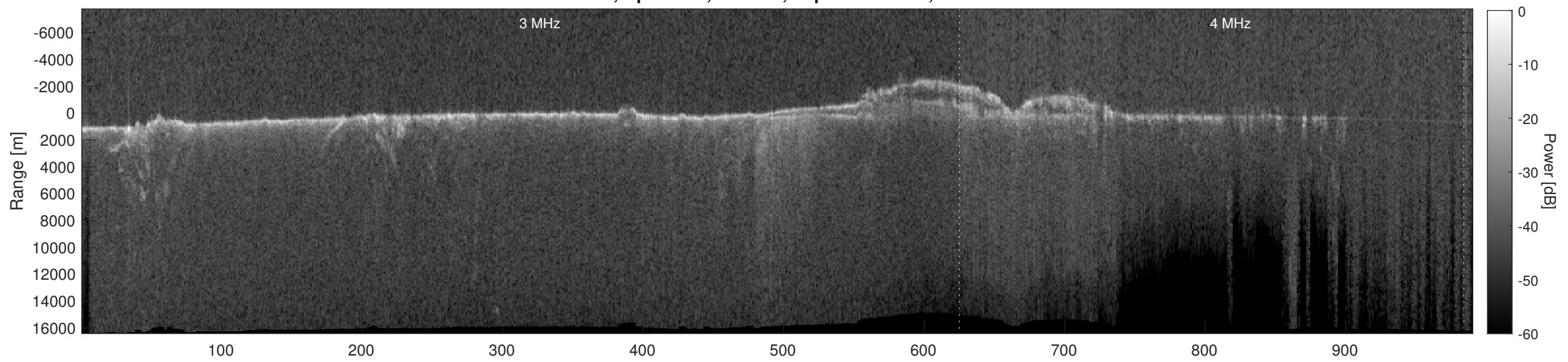
Orbit 9808, Depth-Corrected Cluttergram
