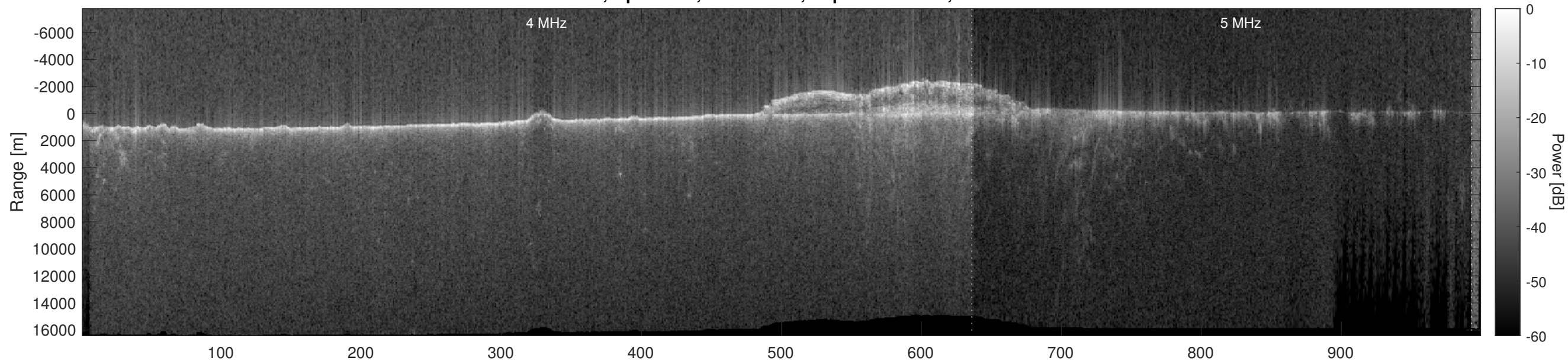
Orbit 9810, Optimized, No Window, Depth-Corrected, Channel 2
