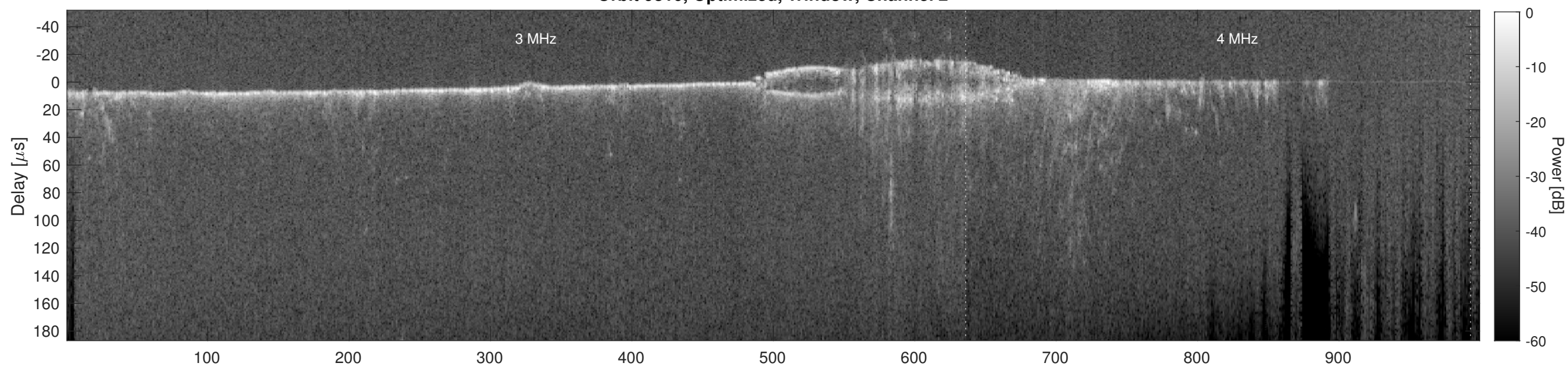
Orbit 9810, Cluttergram
