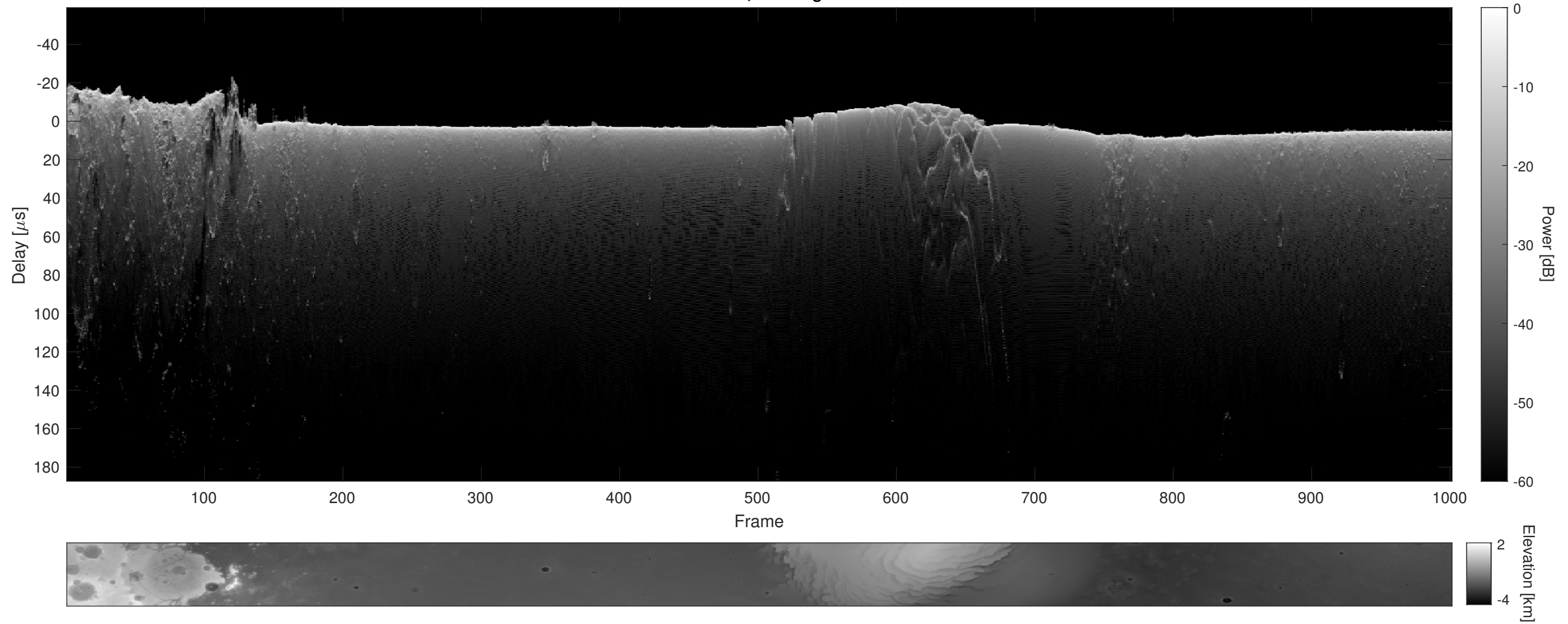
Orbit 9813, Cluttergram
