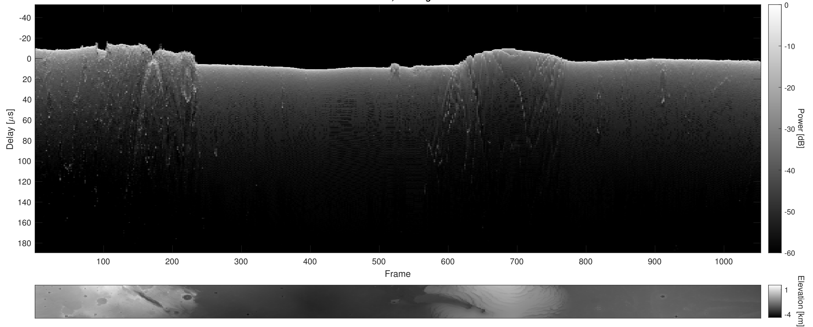
Orbit 9814, Cluttergram
