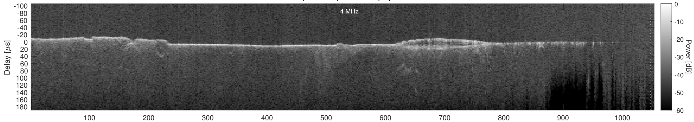
Orbit 9814, Cluttergram
