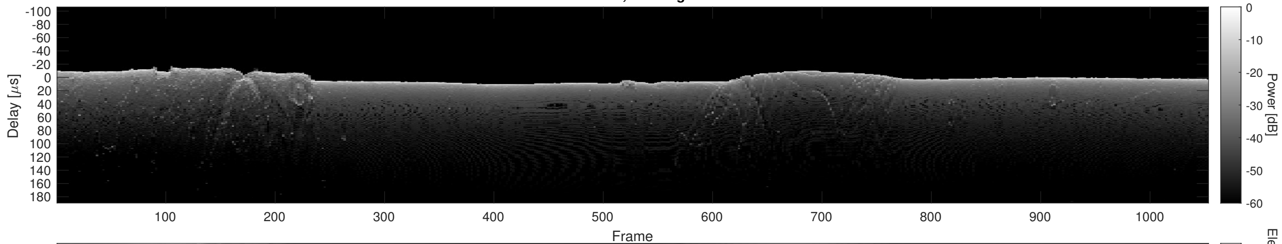
Orbit 9814, Cluttergram
