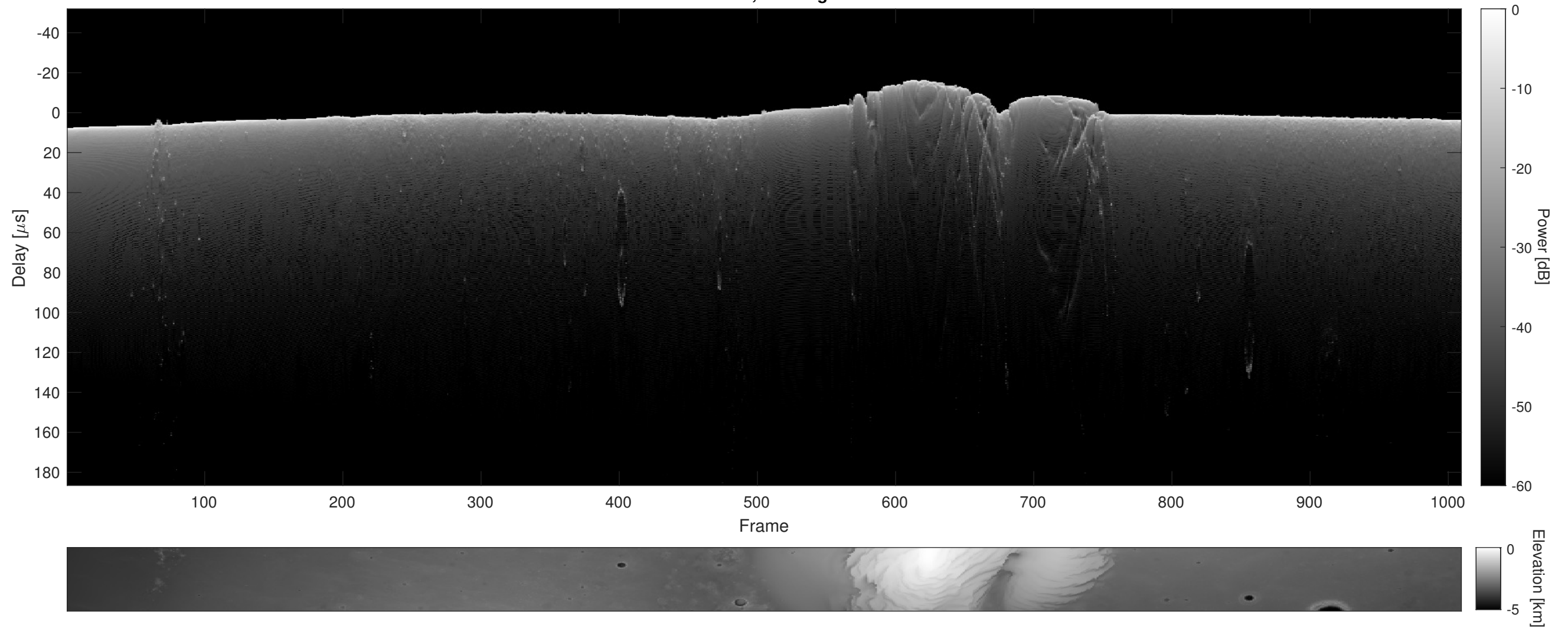
Orbit 9815, Cluttergram
