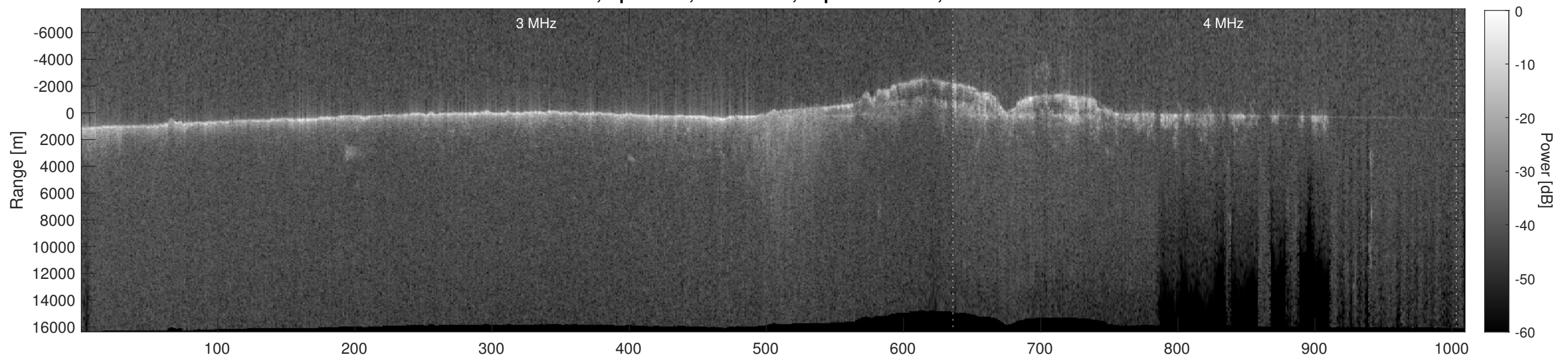
Orbit 9815, Depth-Corrected Cluttergram
