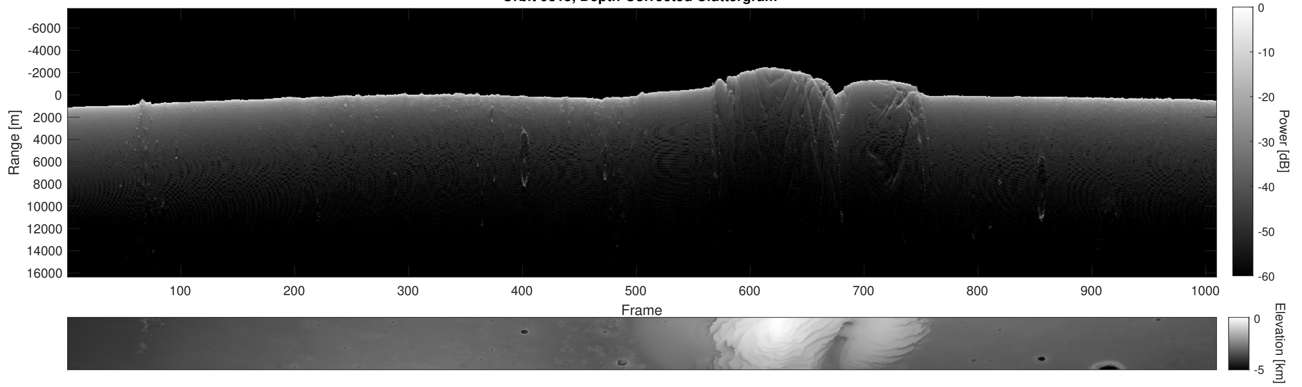
Orbit 9815, Depth-Corrected Cluttergram
