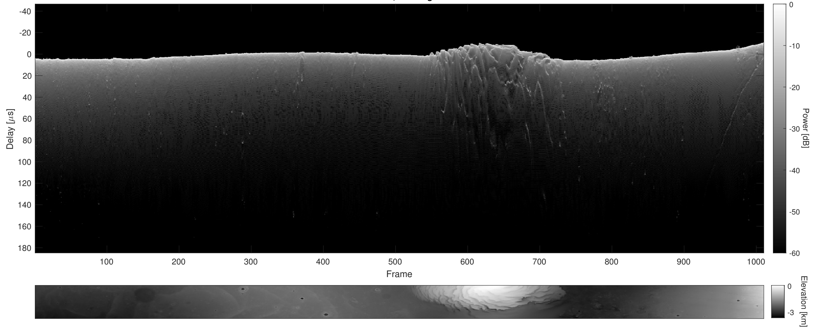
Orbit 9816, Cluttergram
