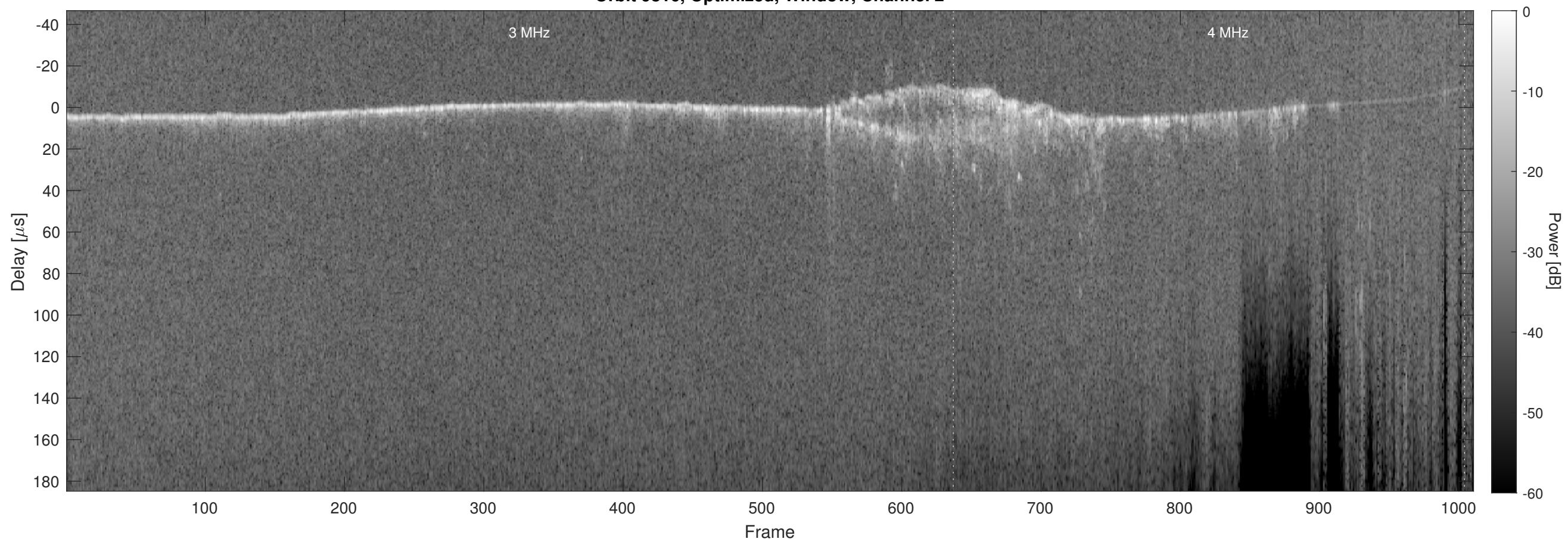
Orbit 9816, Optimized, Window, Channel 2
