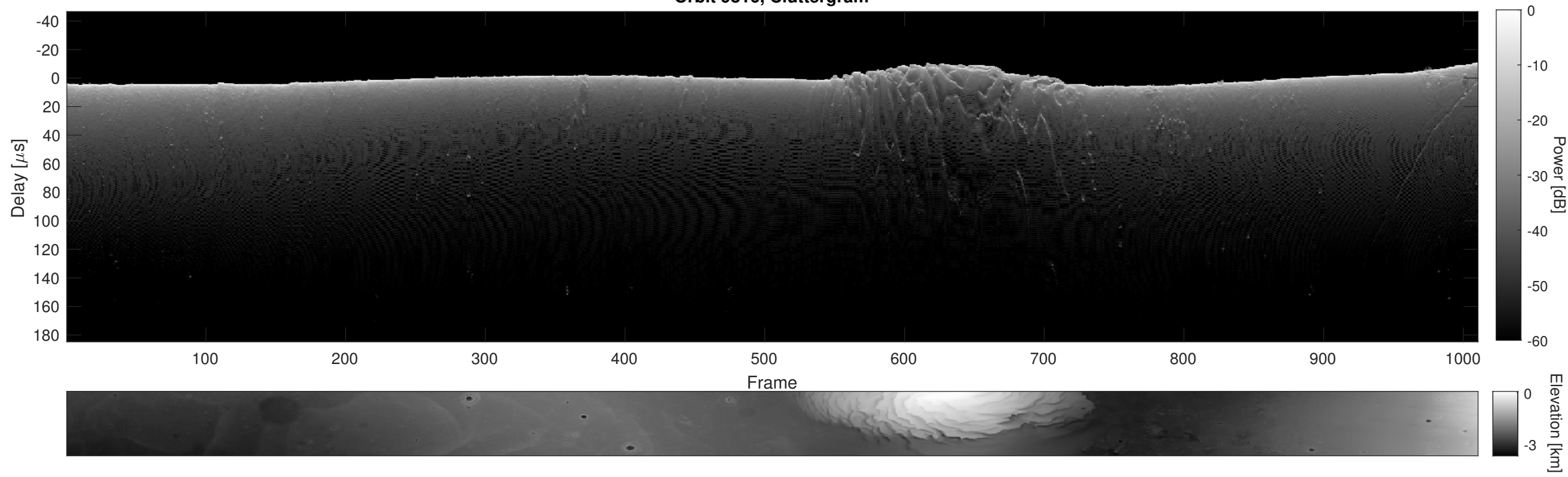
Orbit 9816, Cluttergram
