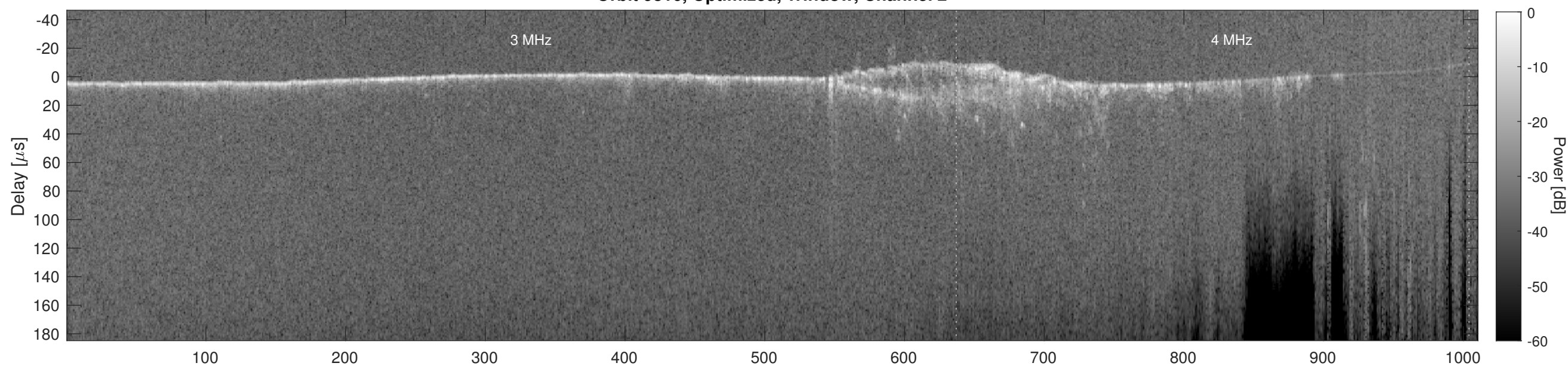
Orbit 9816, Cluttergram
