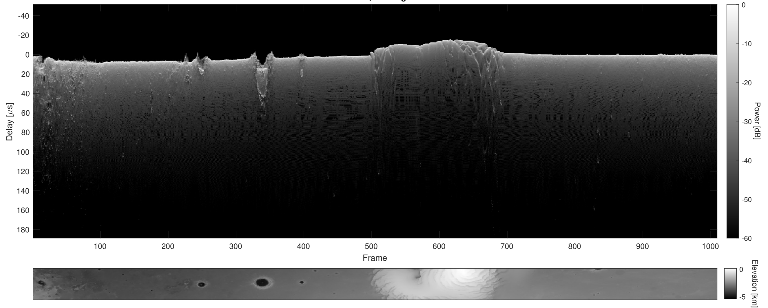
Orbit 9817, Cluttergram
