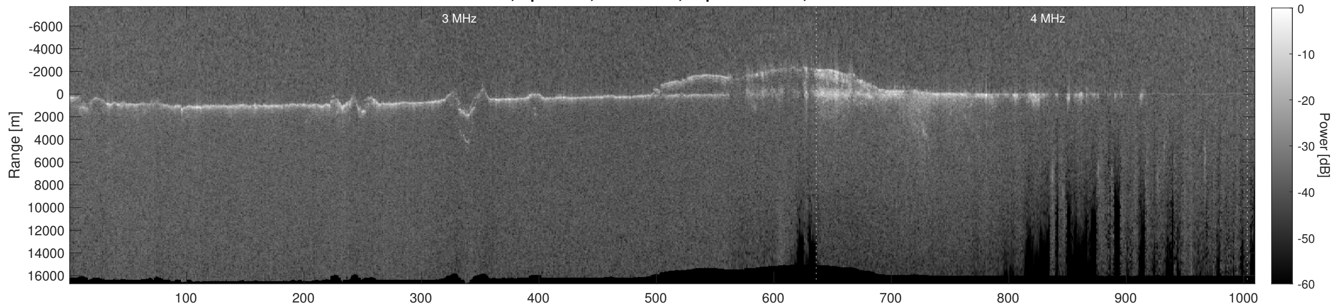
Orbit 9817, Depth-Corrected Cluttergram
