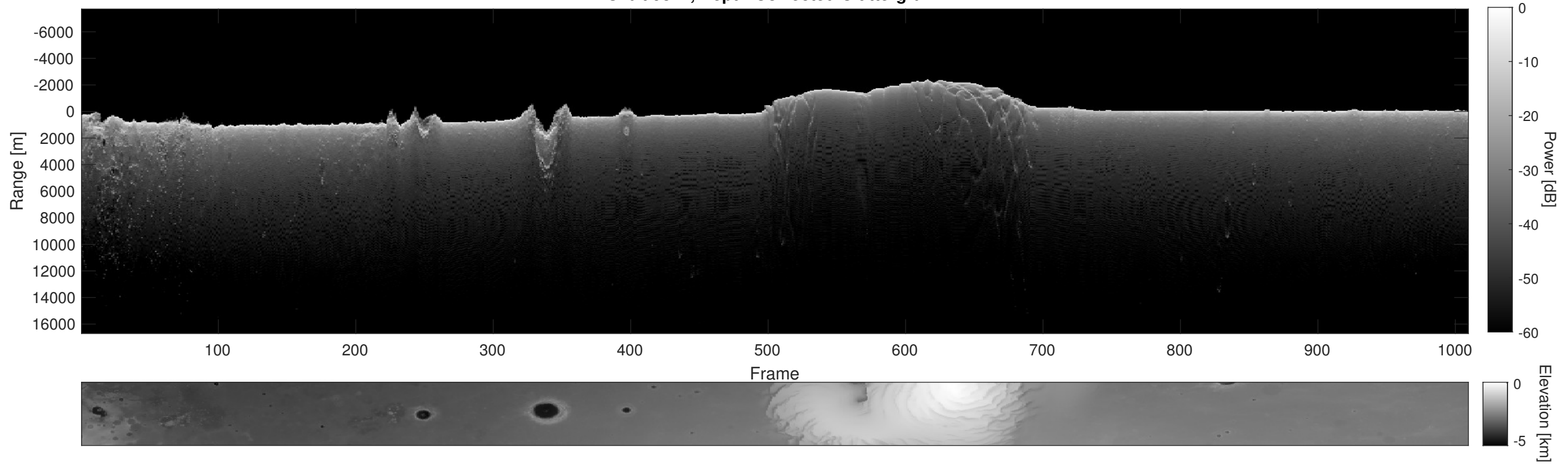
Orbit 9817, Depth-Corrected Cluttergram
