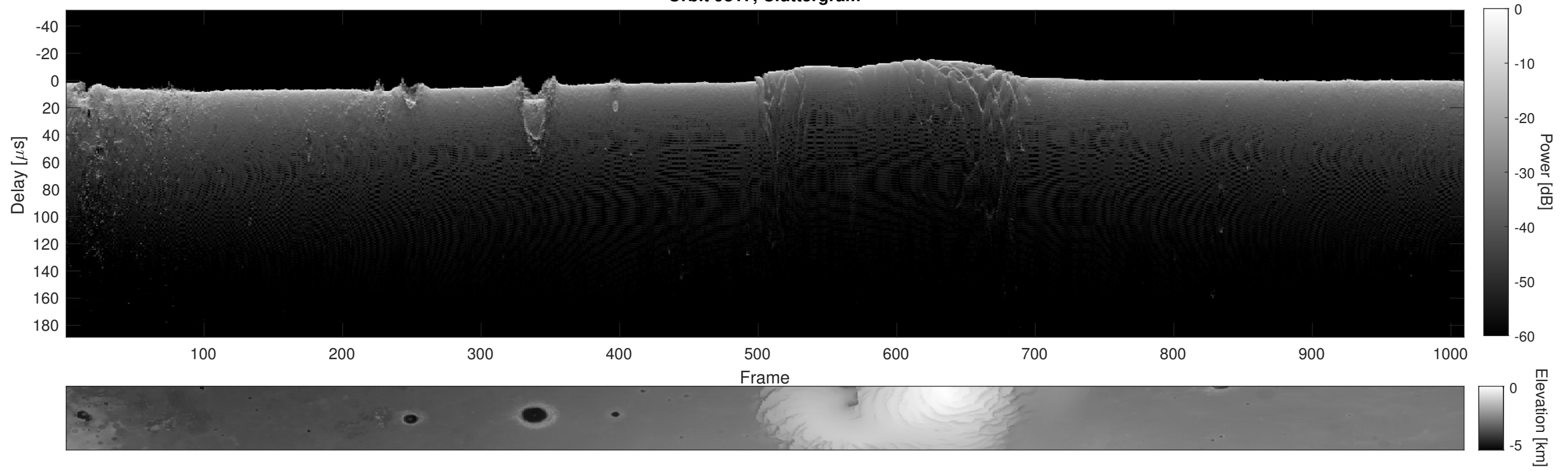
Orbit 9817, Cluttergram
