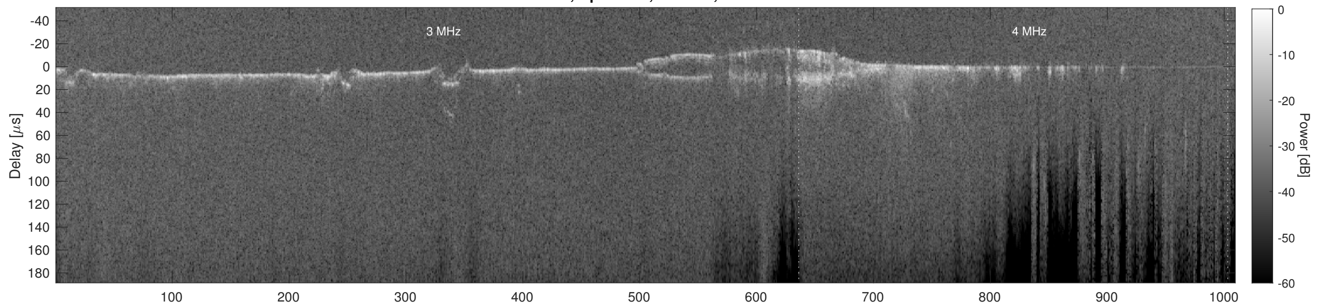
Orbit 9817, Cluttergram
