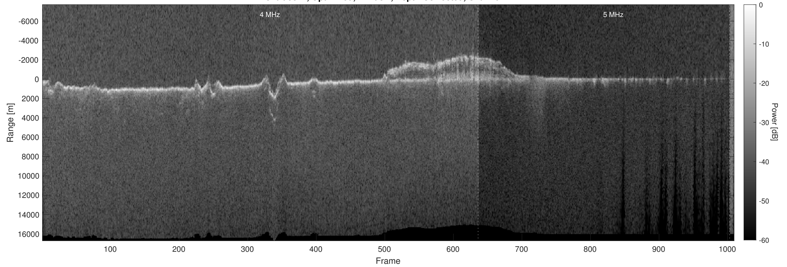
Orbit 9817, Optimized, Window, Depth-Corrected, Channel 2
