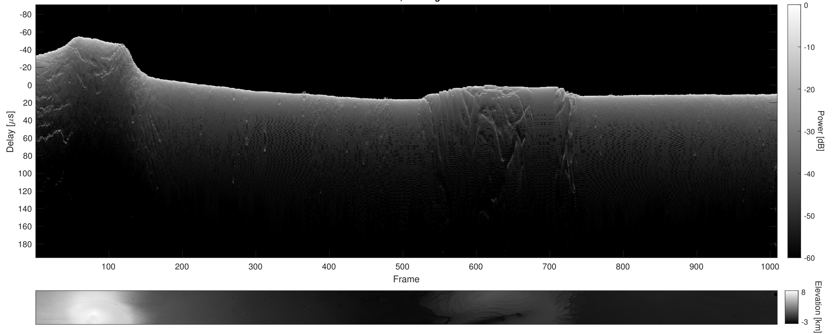
Orbit 9818, Cluttergram
