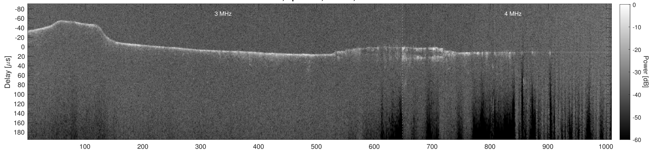
Orbit 9818, Cluttergram
