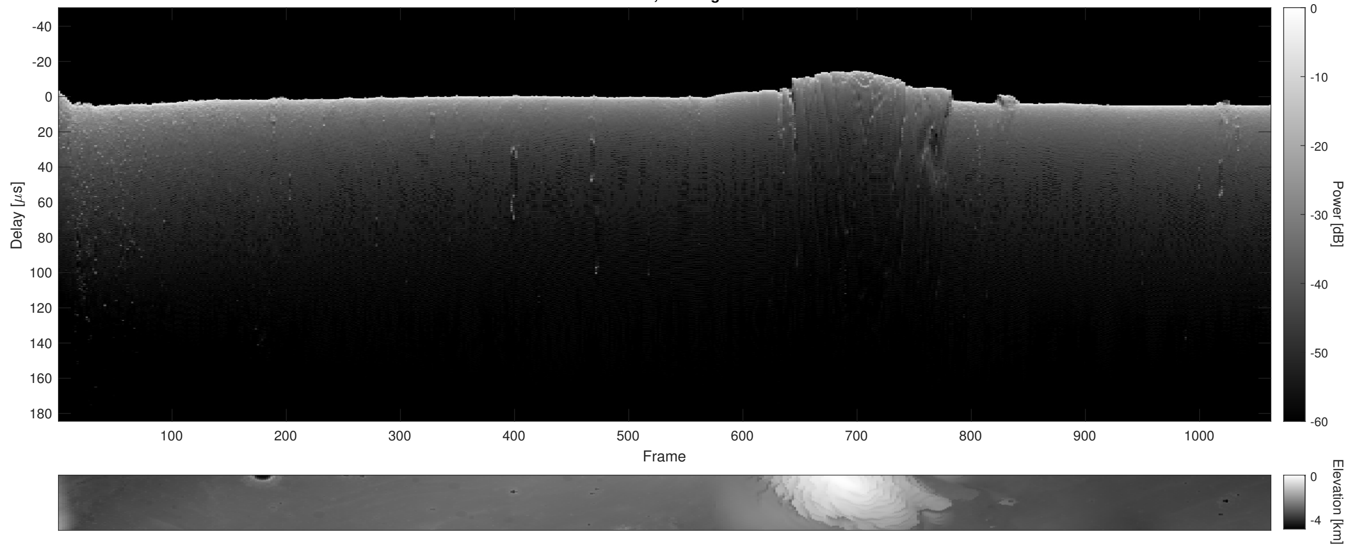
Orbit 9819, Cluttergram
