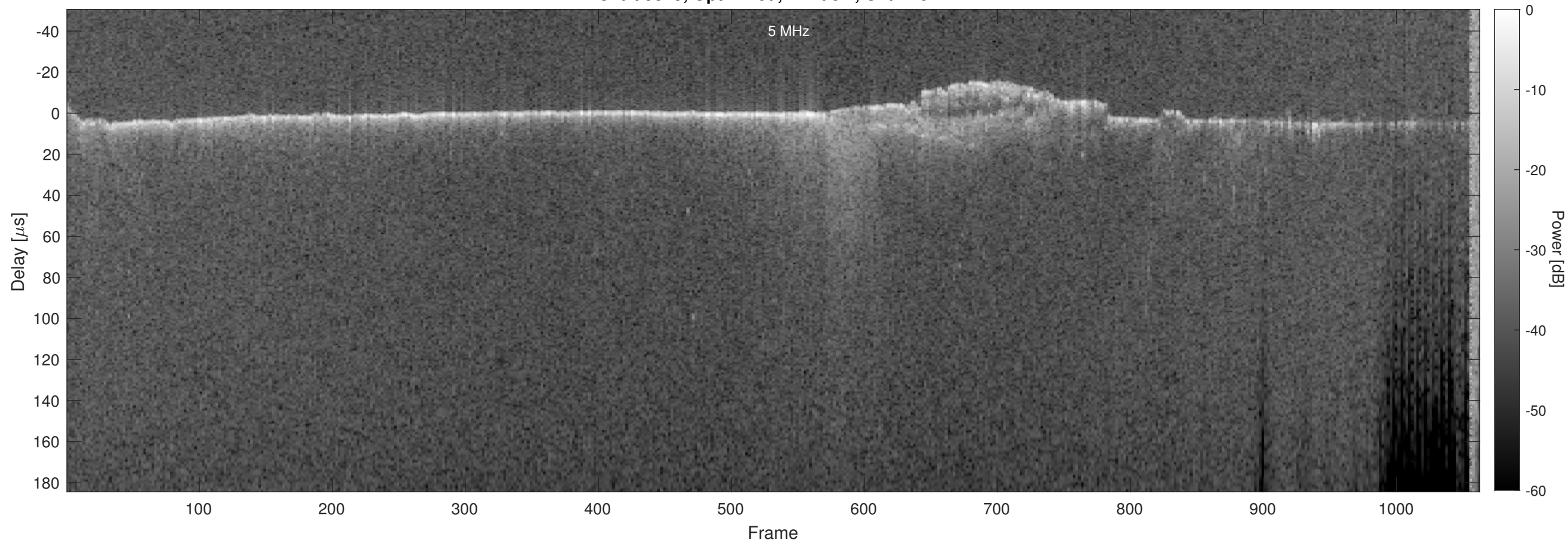
Orbit 9819, Optimized, Window, Channel 2
