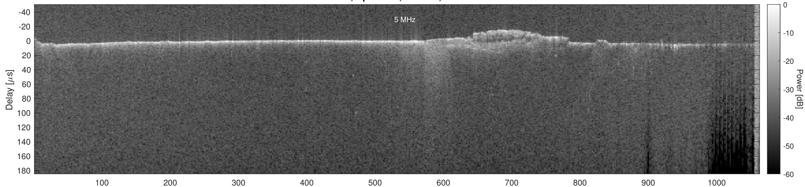
Orbit 9819, Optimized, Window, Channel 2
