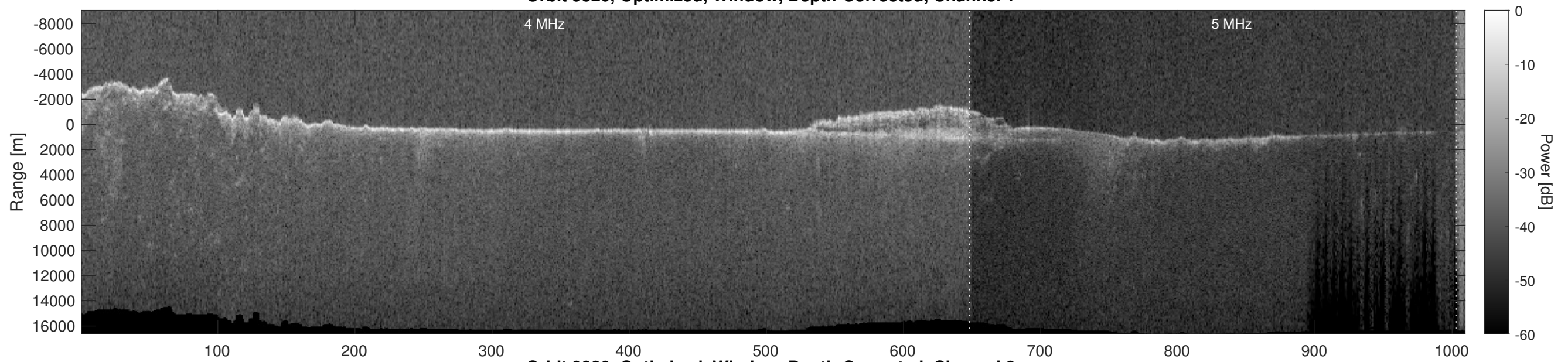
Orbit 9820, Optimized, Window, Depth-Corrected, Channel 2
