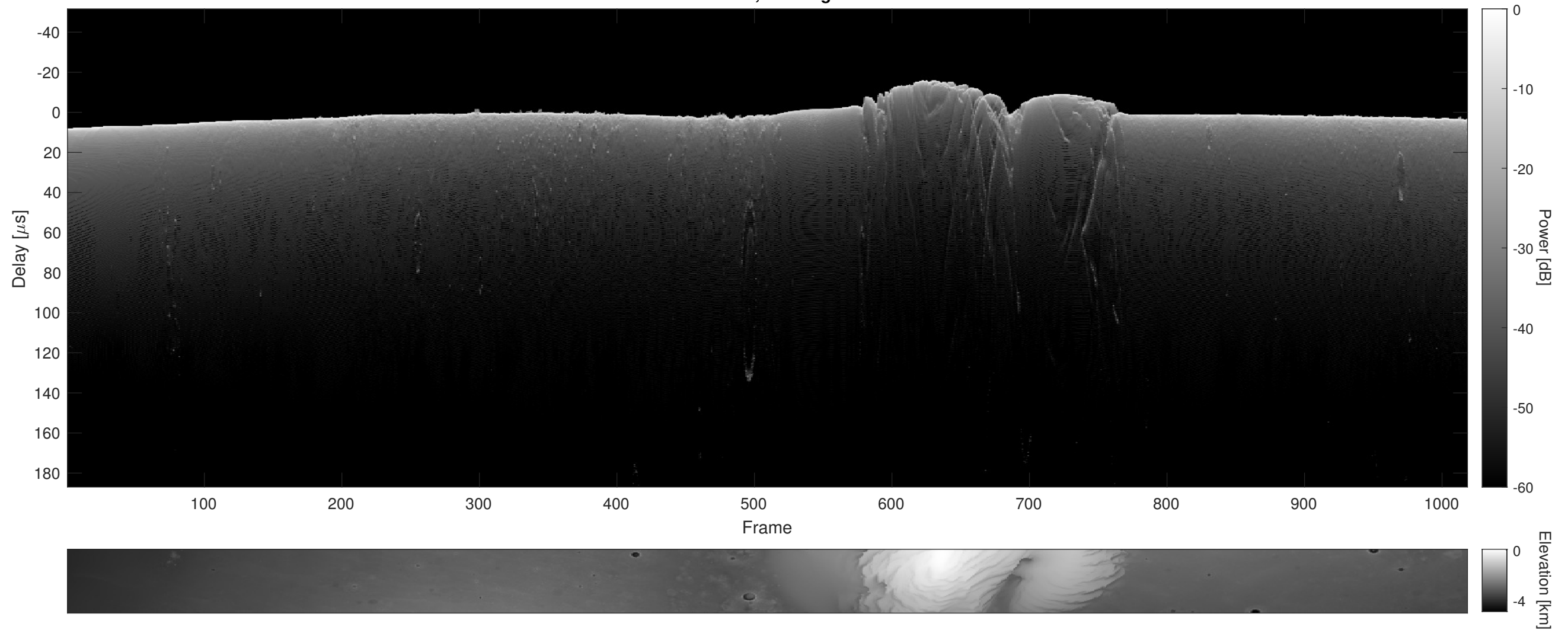
Orbit 9822, Cluttergram
