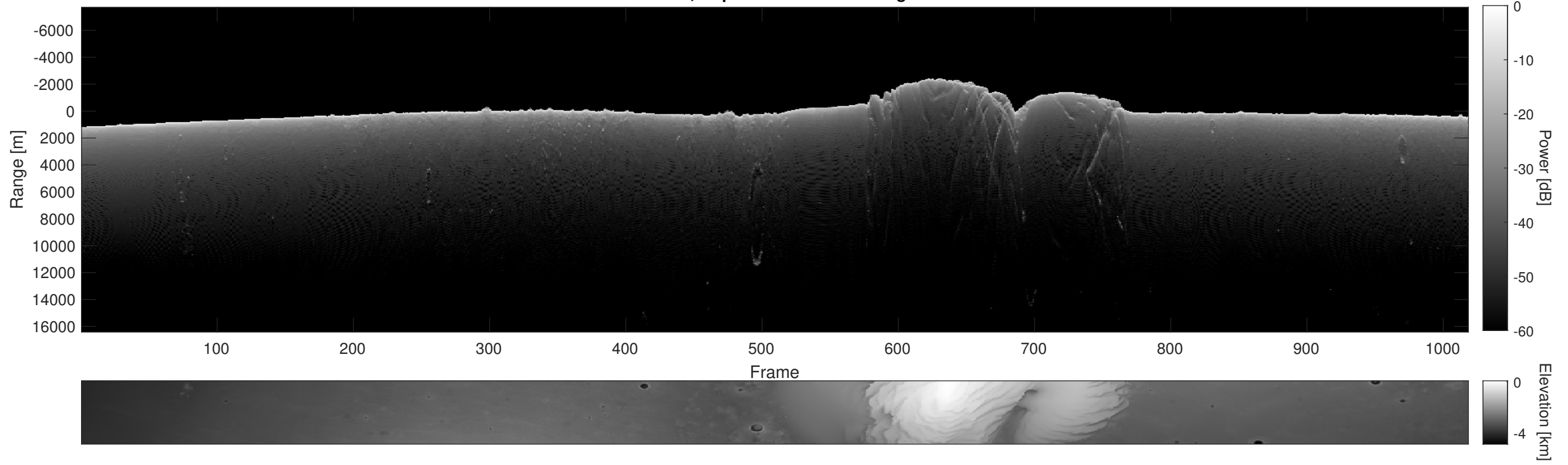
Orbit 9822, Depth-Corrected Cluttergram
