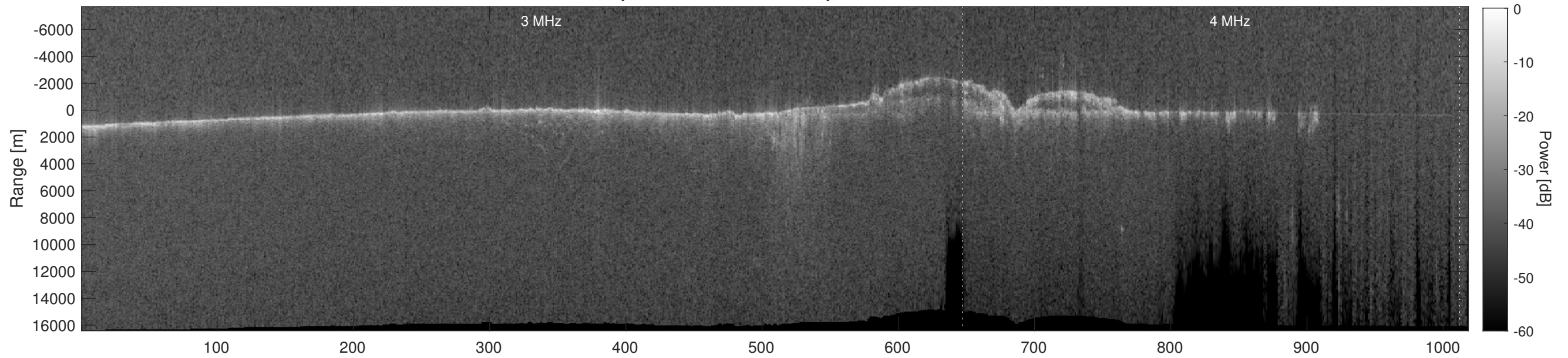
Orbit 9822, Depth-Corrected Cluttergram
