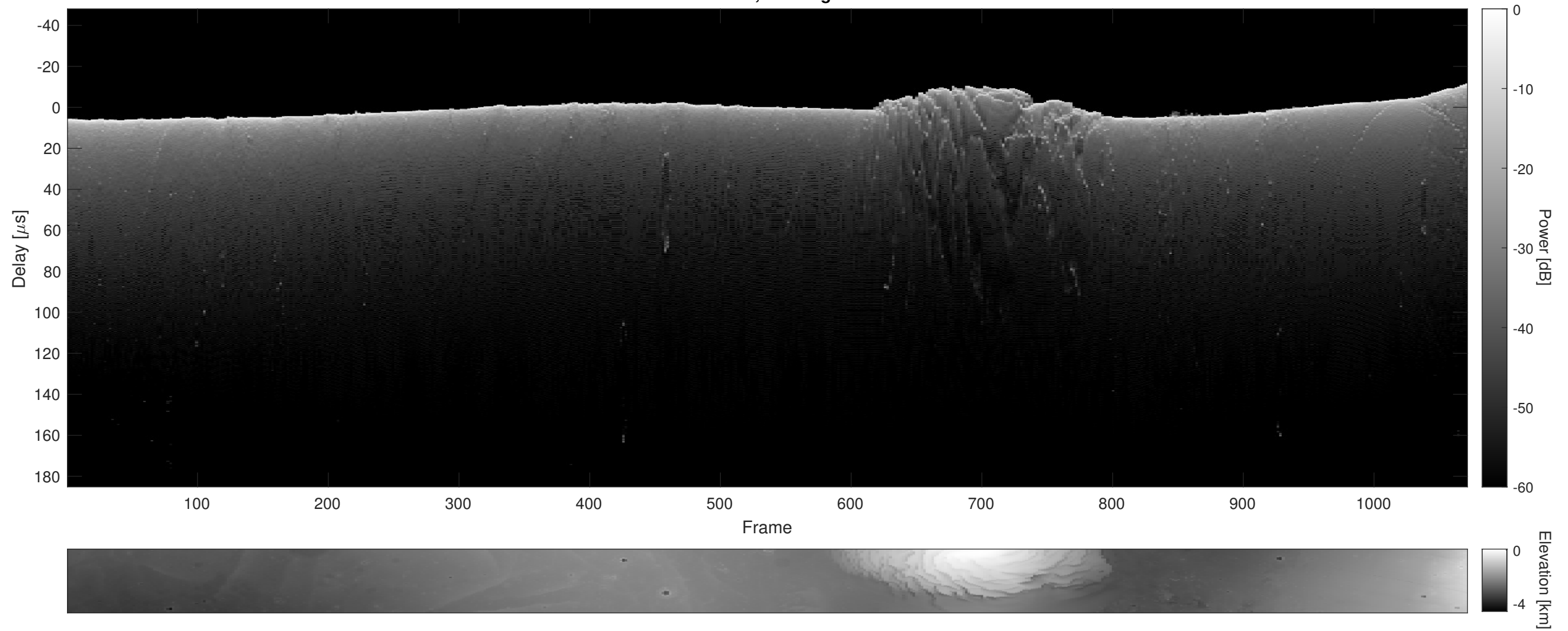
Orbit 9823, Cluttergram
