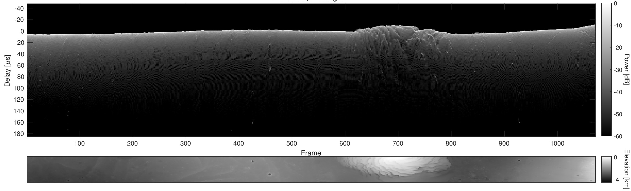
Orbit 9823, Cluttergram
