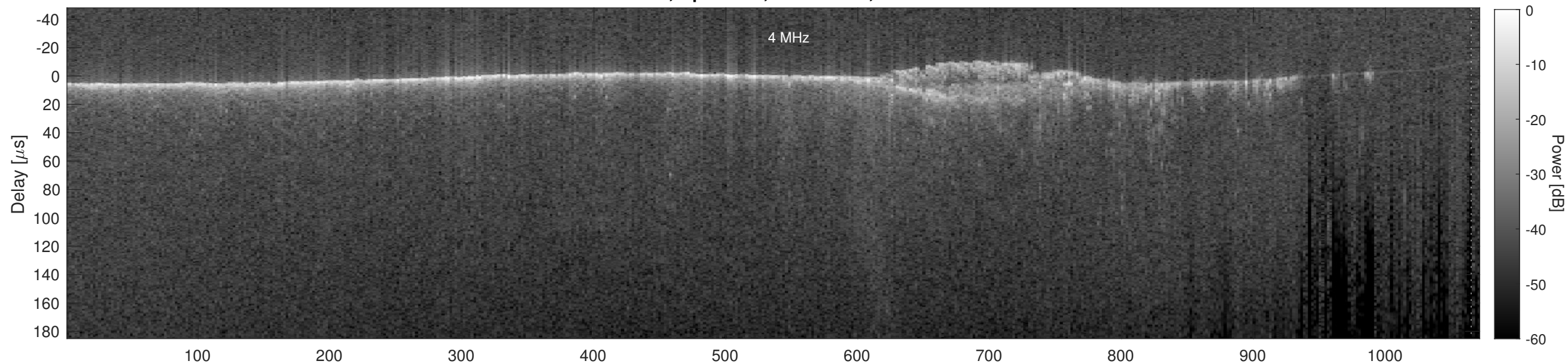
Orbit 9823, Cluttergram
