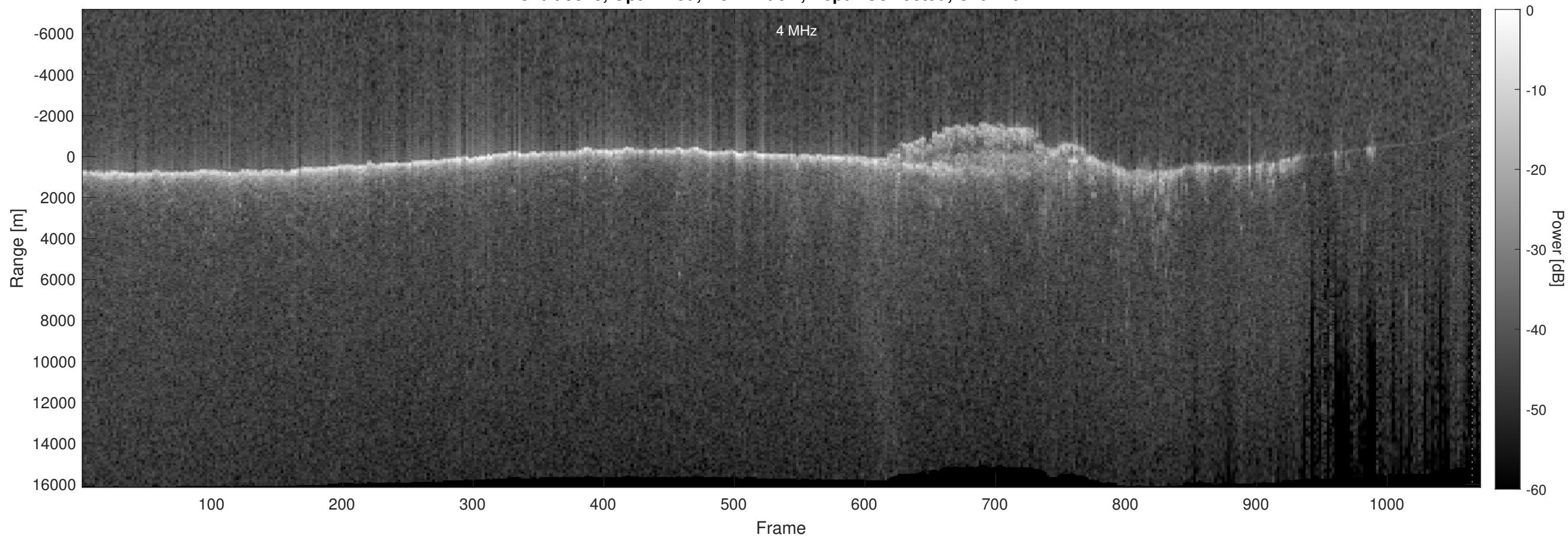
Orbit 9823, Optimized, No Window, Depth-Corrected, Channel 2
