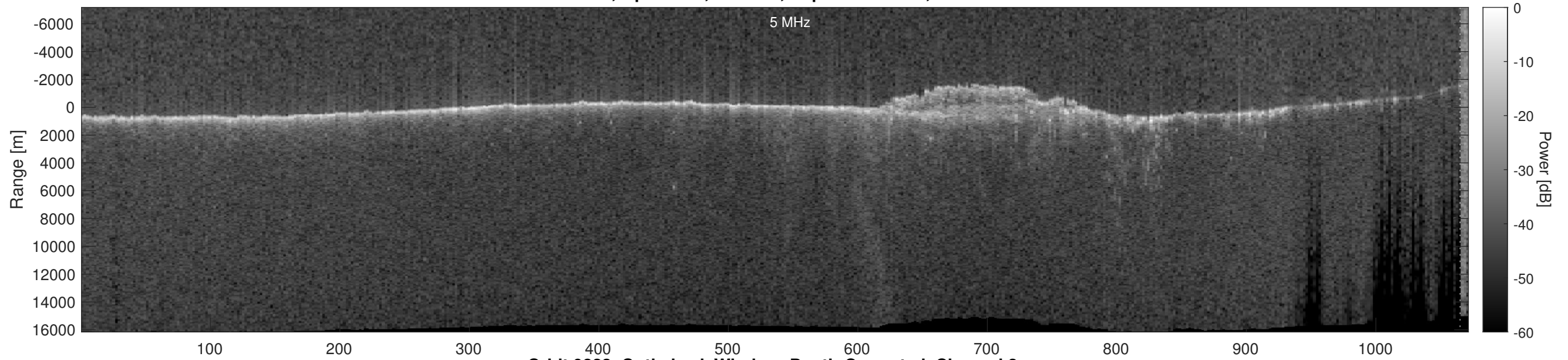
Orbit 9823, Optimized, Window, Depth-Corrected, Channel 2
