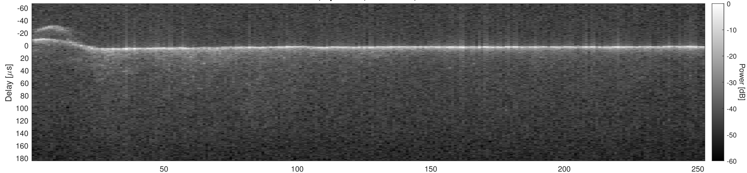
Orbit 9826, Optimized, No Window, Channel 2
