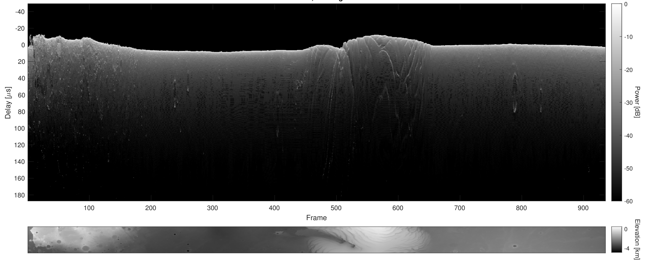
Orbit 9828, Cluttergram
