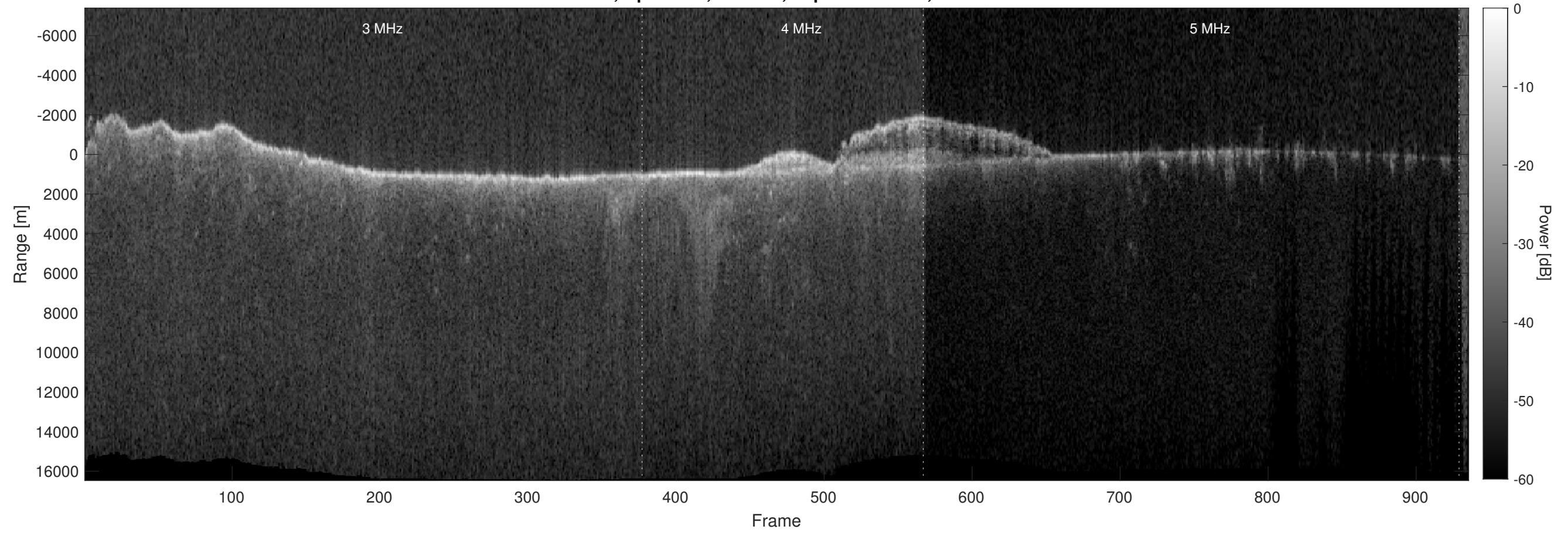
Orbit 9828, Optimized, Window, Depth-Corrected, Channel 2
