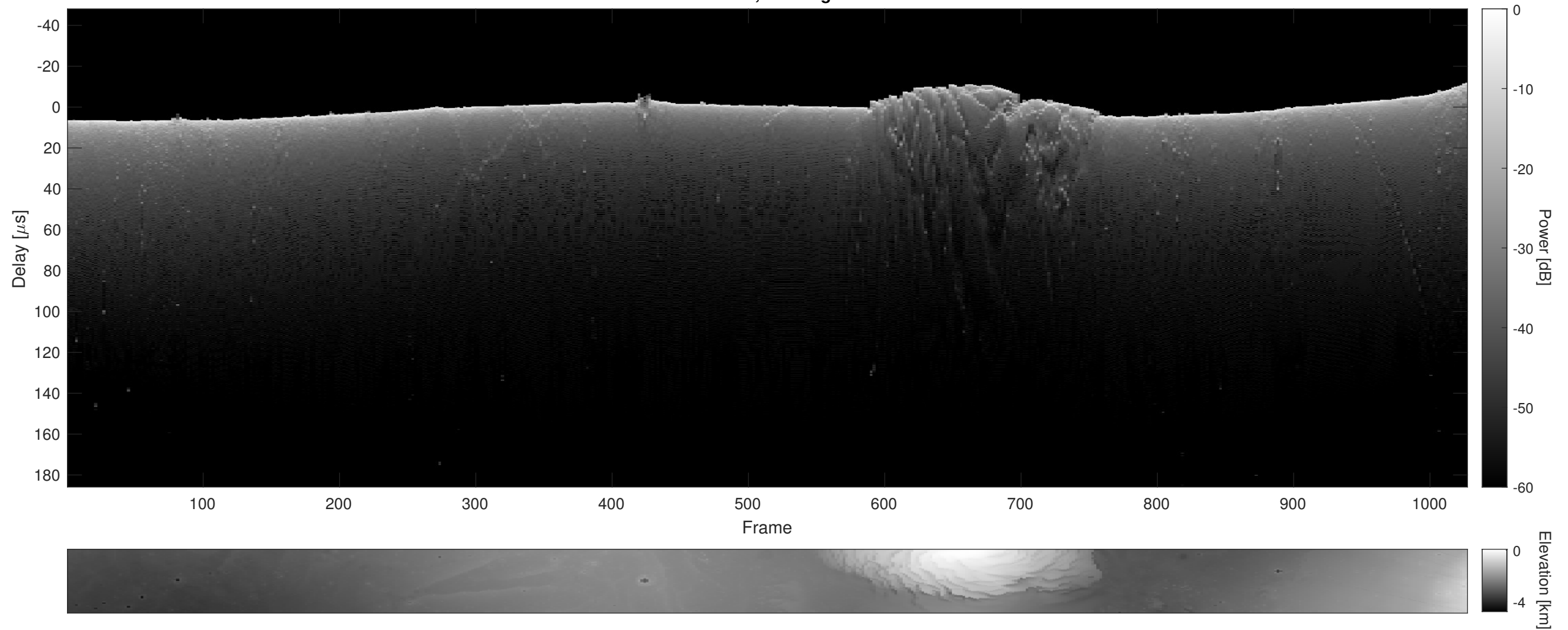
Orbit 9830, Cluttergram
