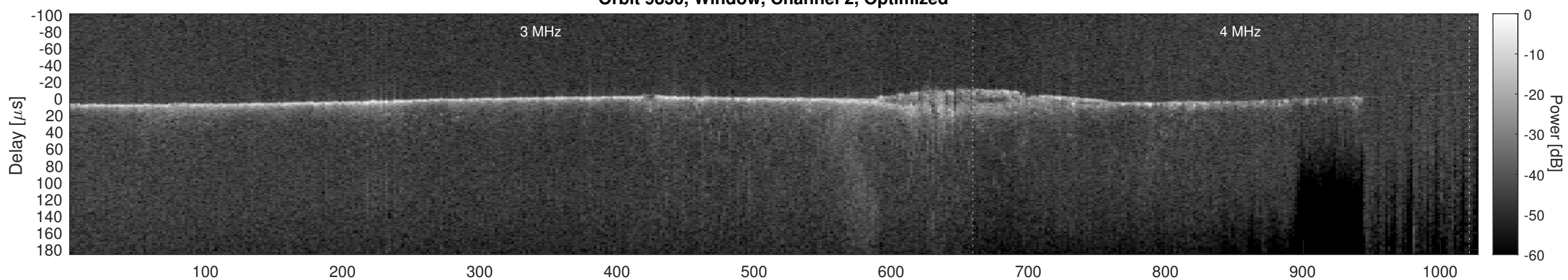
Orbit 9830, Cluttergram
