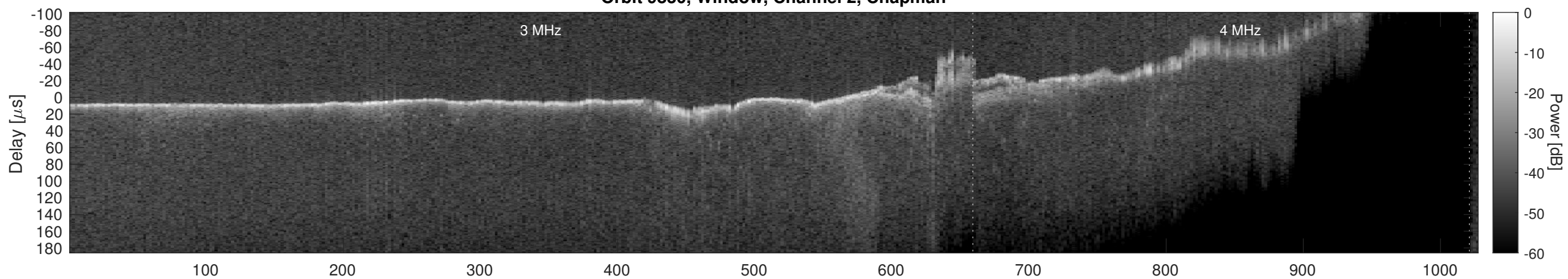
Orbit 9830, Window, Channel 2, Optimized
