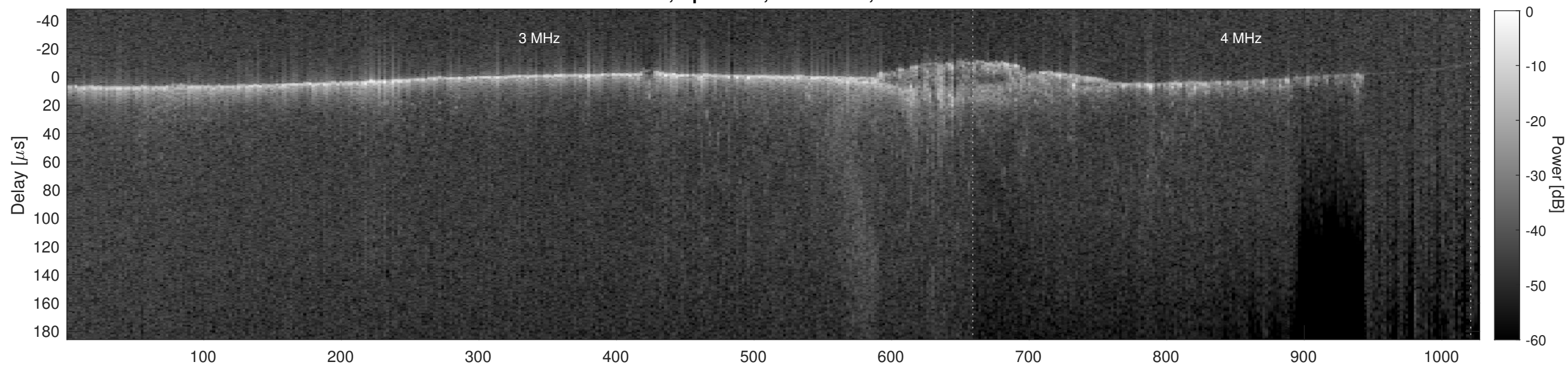
Orbit 9830, Cluttergram
