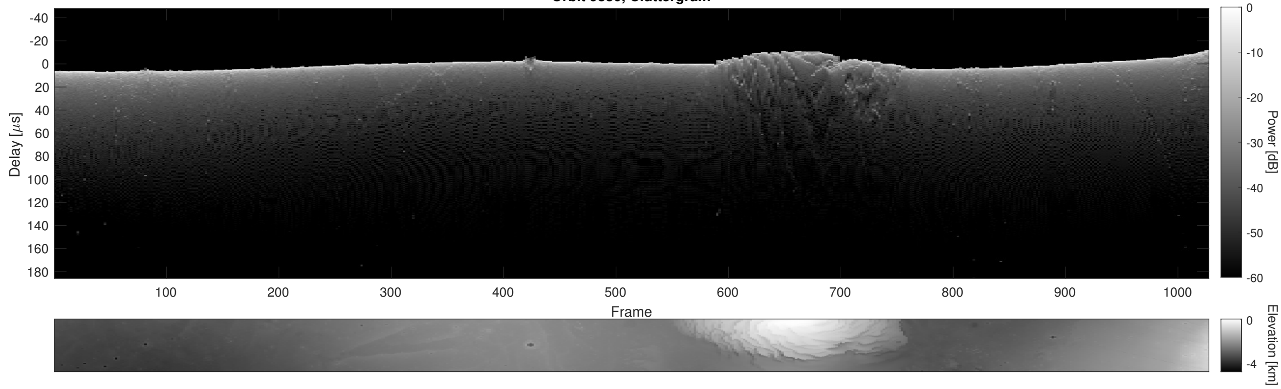
Orbit 9830, Cluttergram
