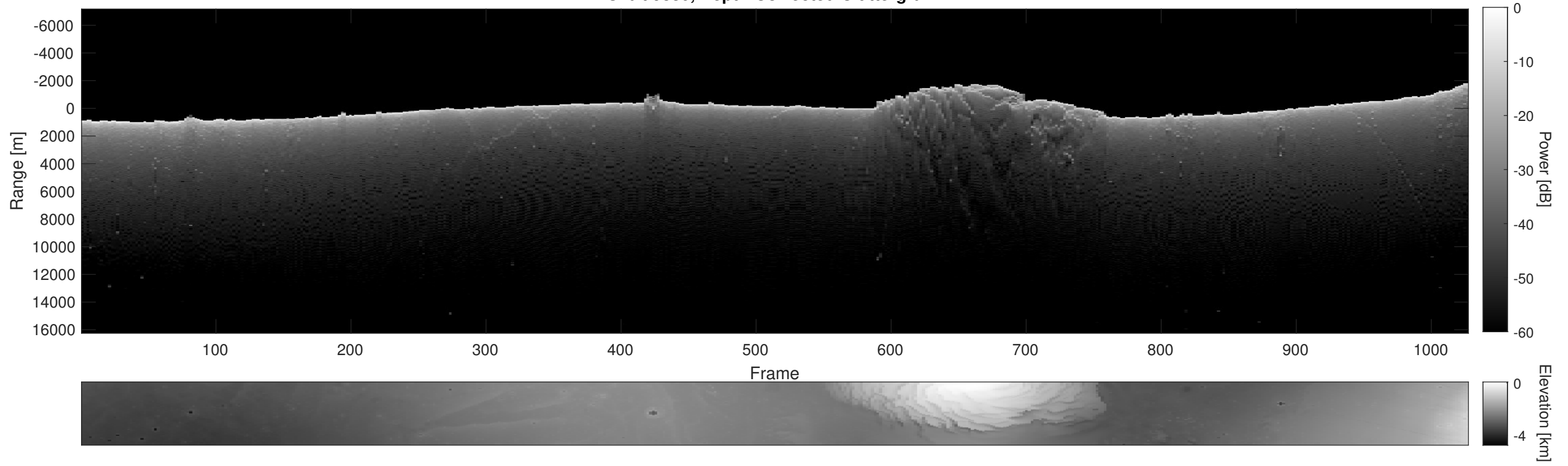
Orbit 9830, Depth-Corrected Cluttergram
