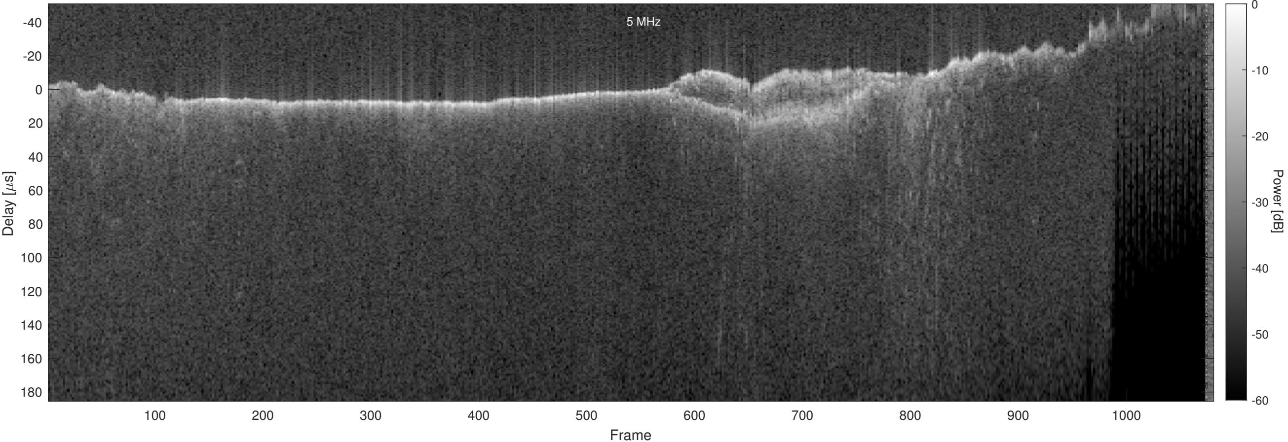
Orbit 9831, Chapman, Window, Channel 2
