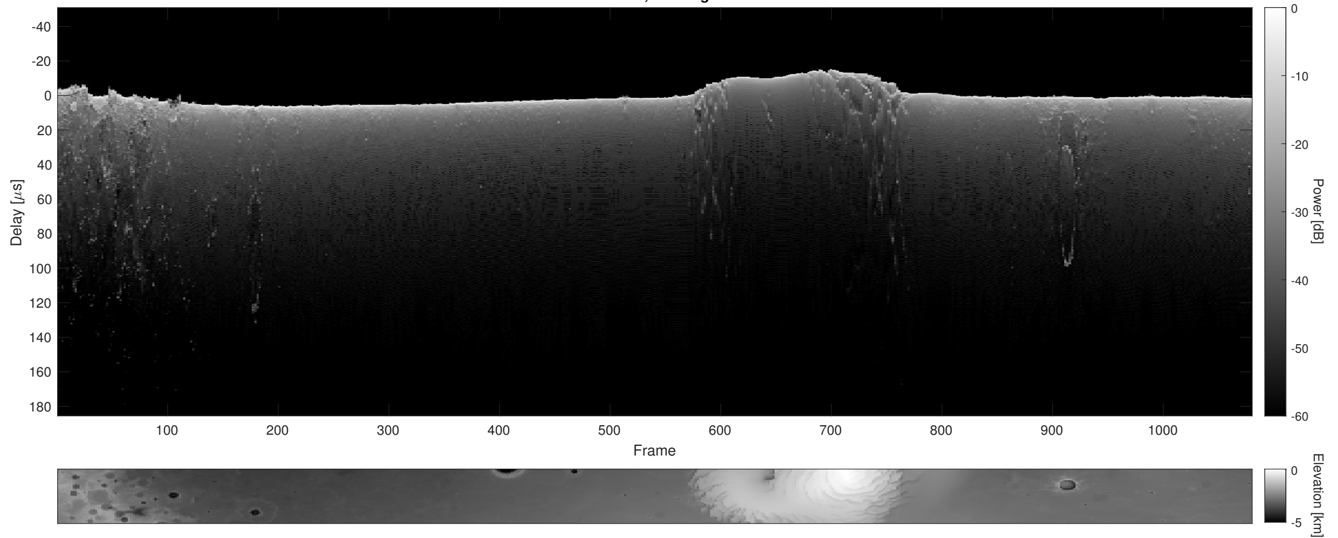
Orbit 9831, Cluttergram
