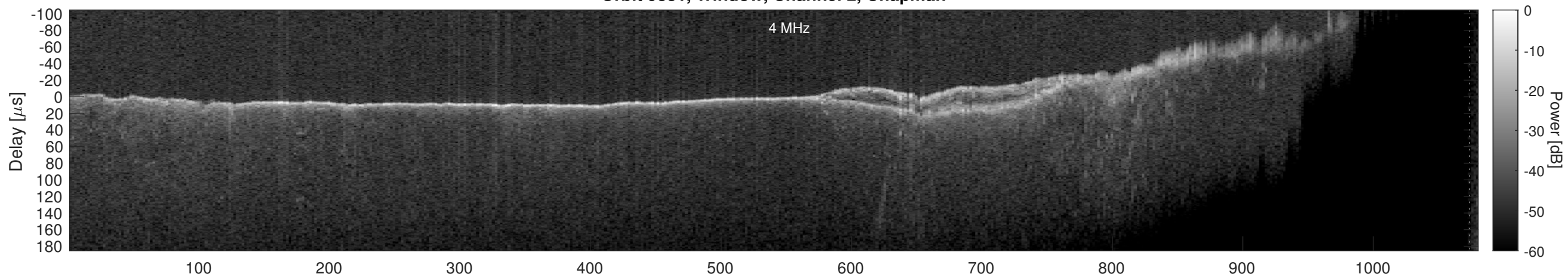
Orbit 9831, Window, Channel 2, Optimized
