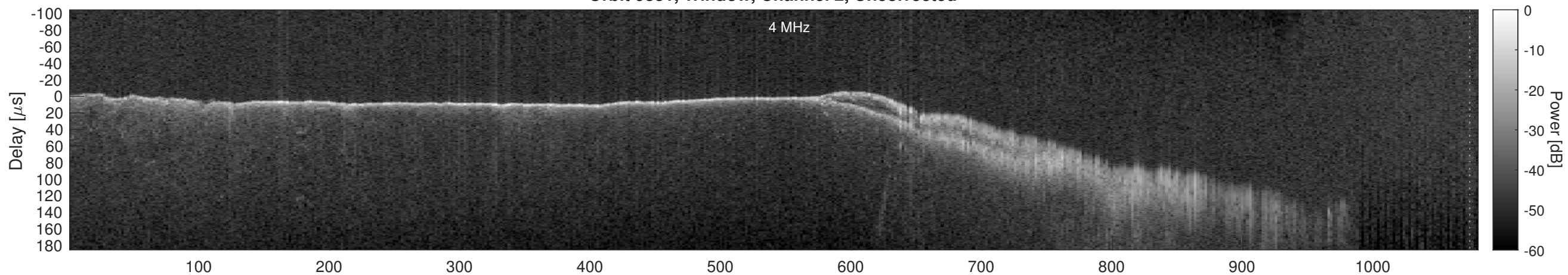
Orbit 9831, Window, Channel 2, Chapman
