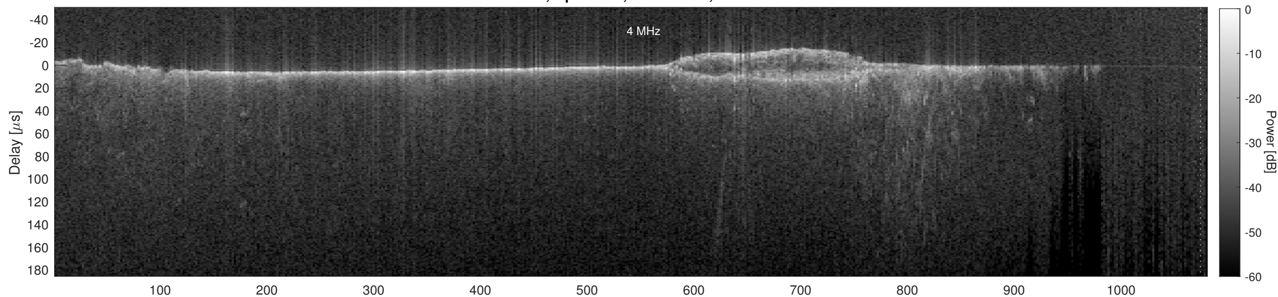
Orbit 9831, Cluttergram
