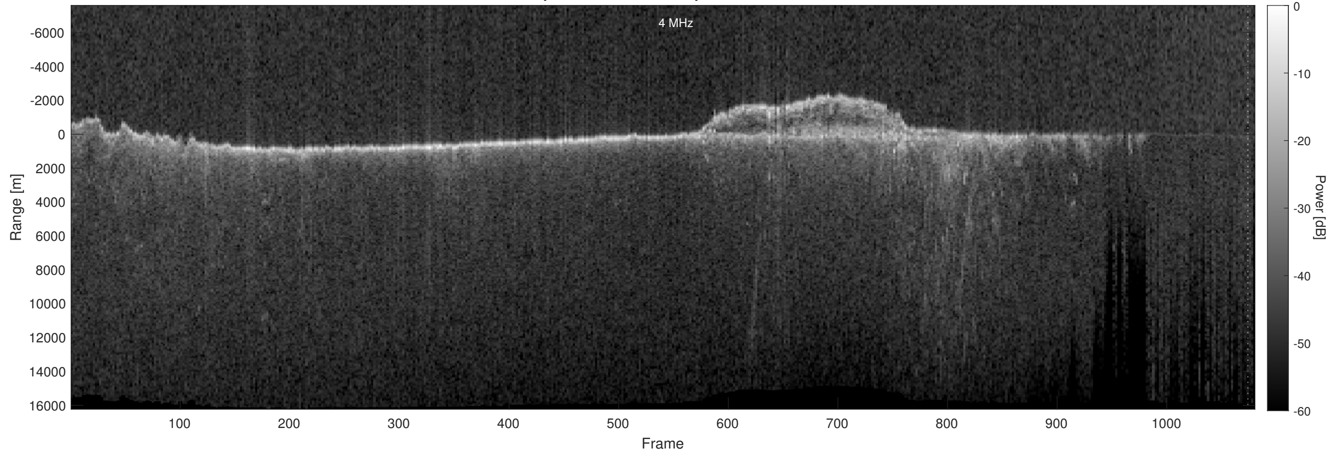
Orbit 9831, Optimized, Window, Depth-Corrected, Channel 2
