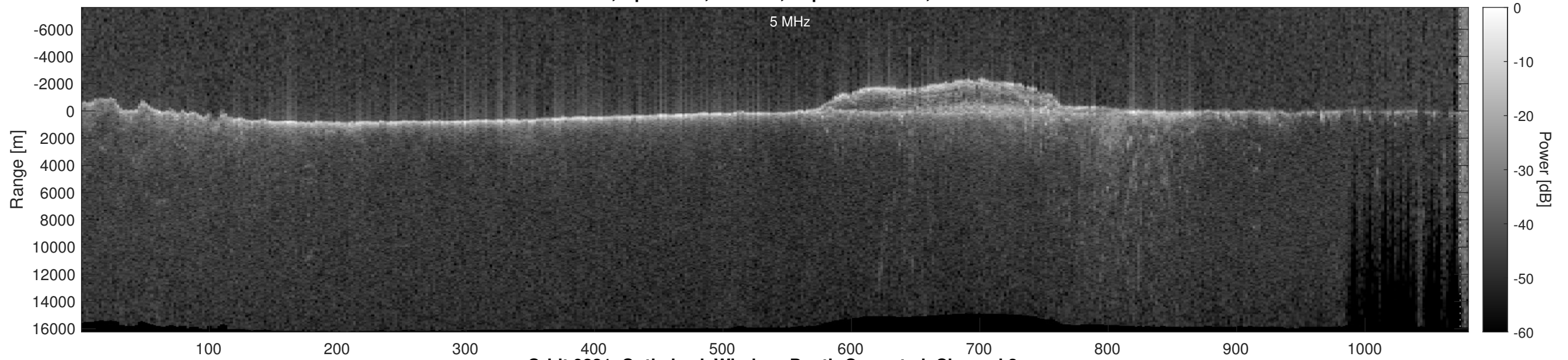
Orbit 9831, Optimized, Window, Depth-Corrected, Channel 2
