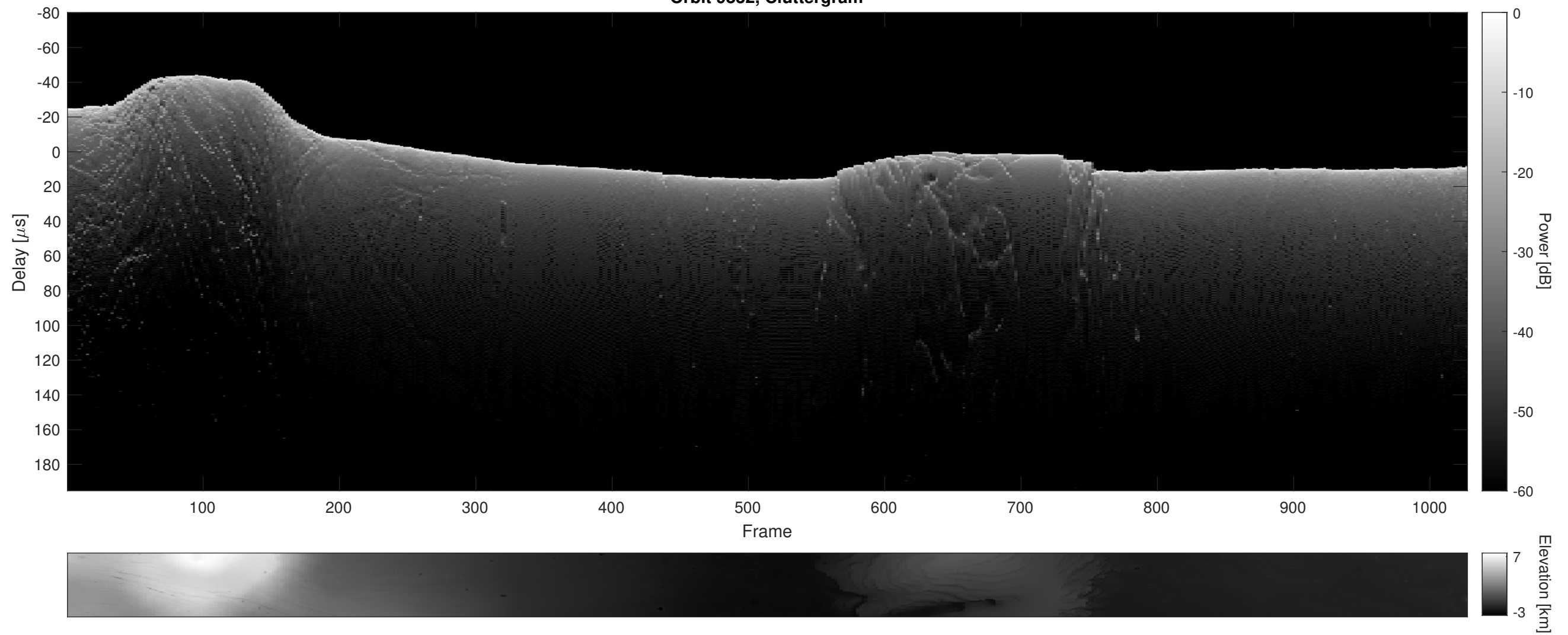
Orbit 9832, Cluttergram
