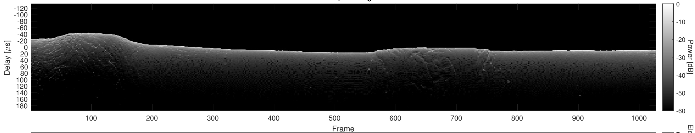
Orbit 9832, Cluttergram
