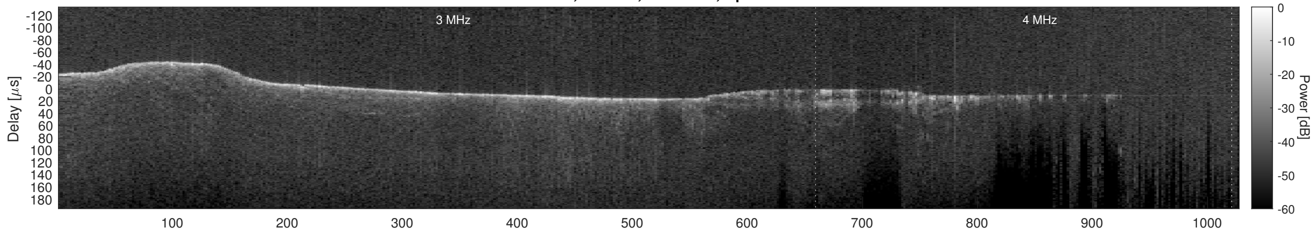
Orbit 9832, Cluttergram
