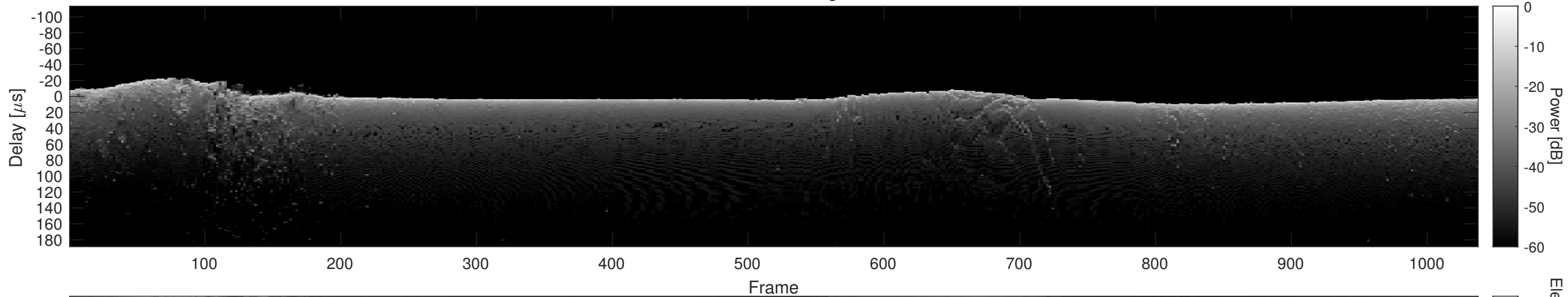
Orbit 9834, Cluttergram
