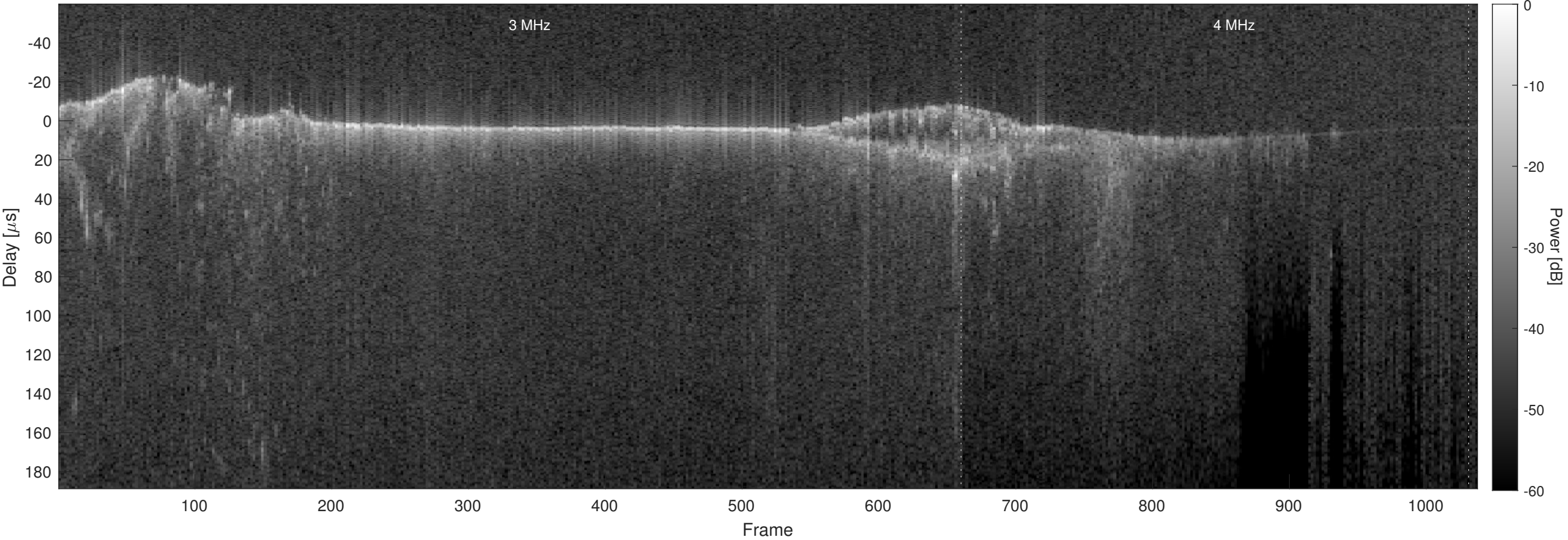
Orbit 9834, Optimized, No Window, Channel 2
