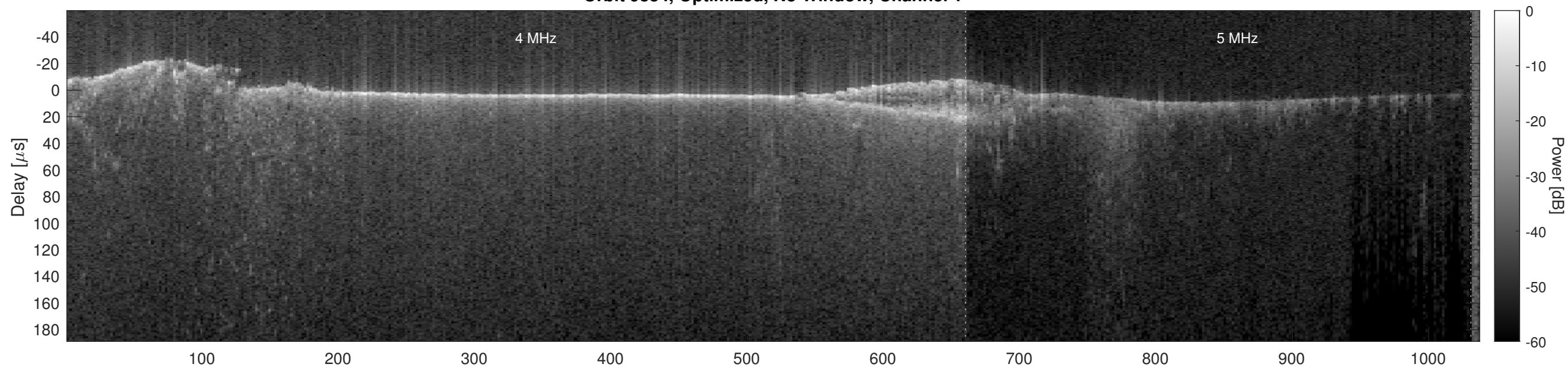
Orbit 9834, Optimized, No Window, Channel 2
