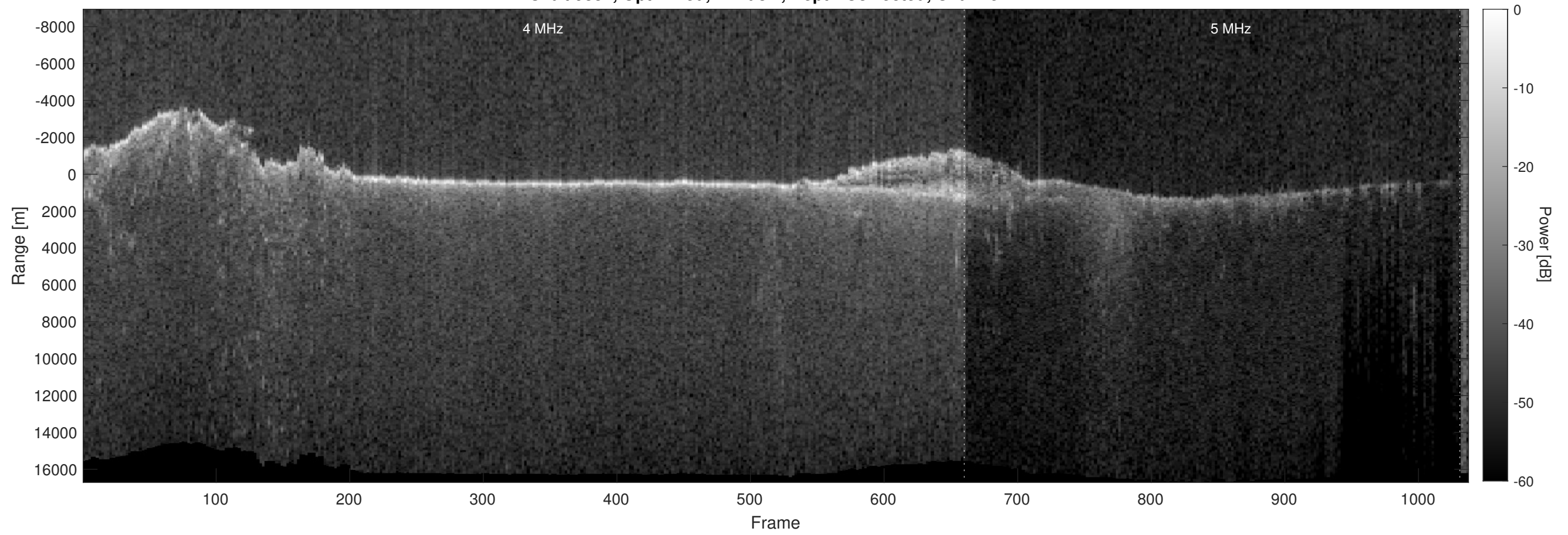
Orbit 9834, Optimized, Window, Depth-Corrected, Channel 2
