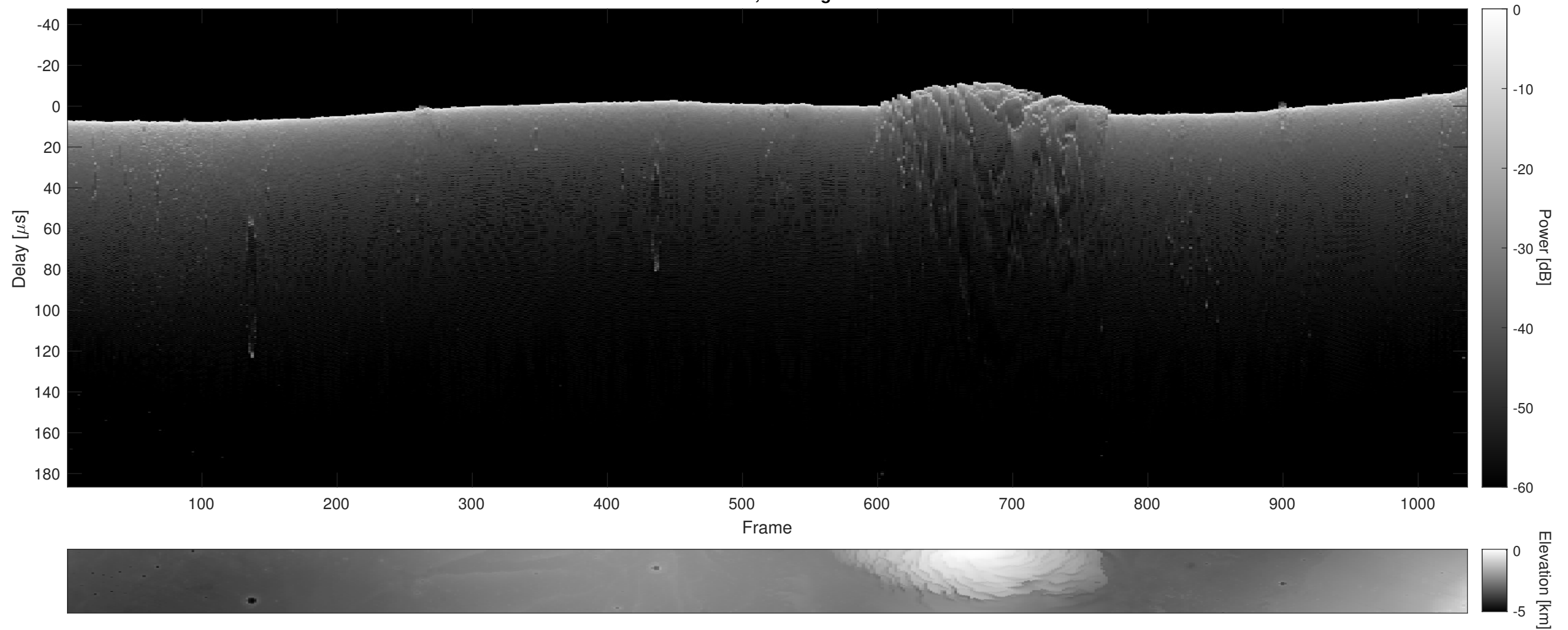
Orbit 9837, Cluttergram
