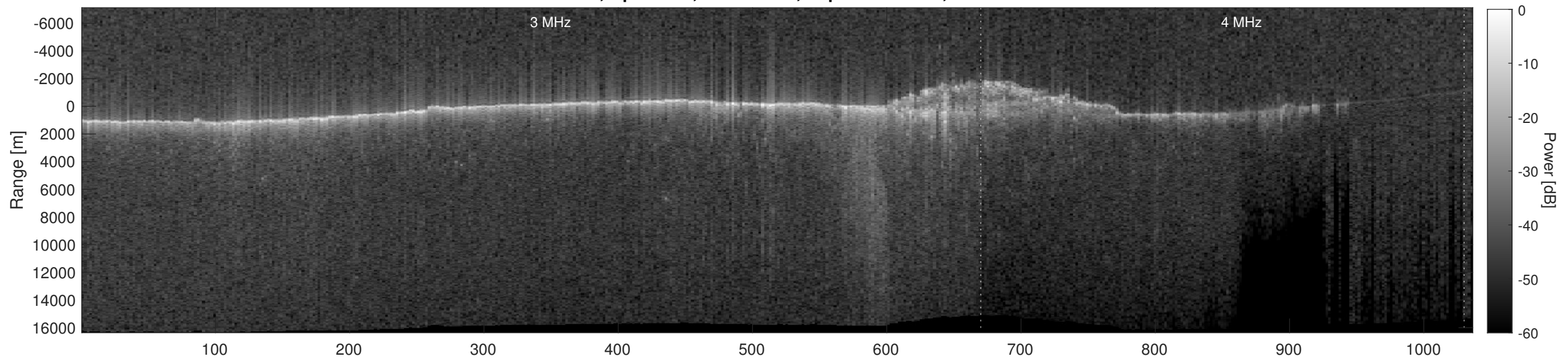
Orbit 9837, Depth-Corrected Cluttergram
