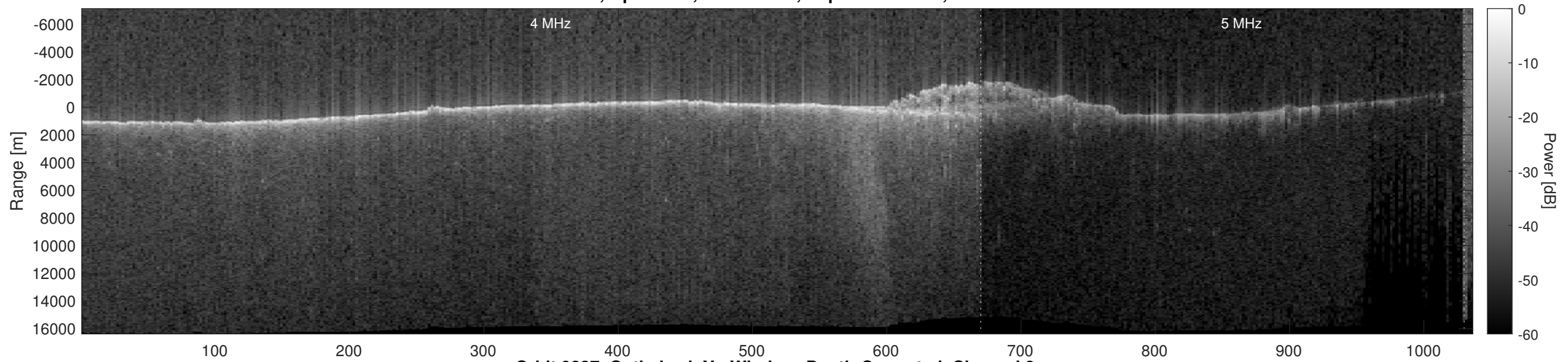
Orbit 9837, Optimized, No Window, Depth-Corrected, Channel 2
