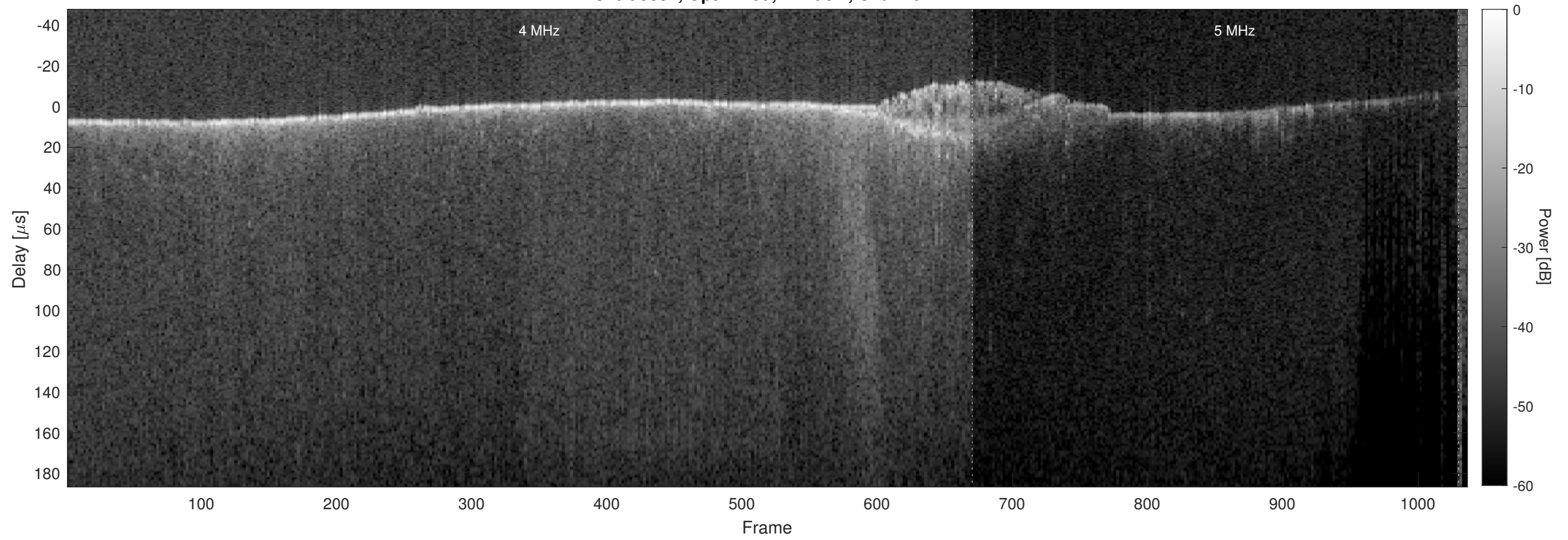
Orbit 9837, Optimized, Window, Channel 2
