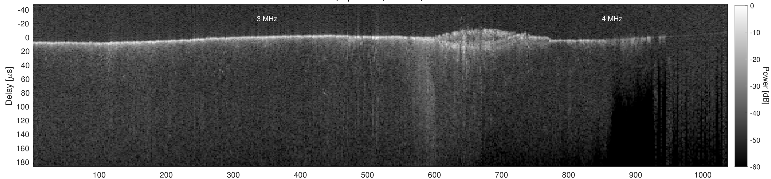
Orbit 9837, Cluttergram
