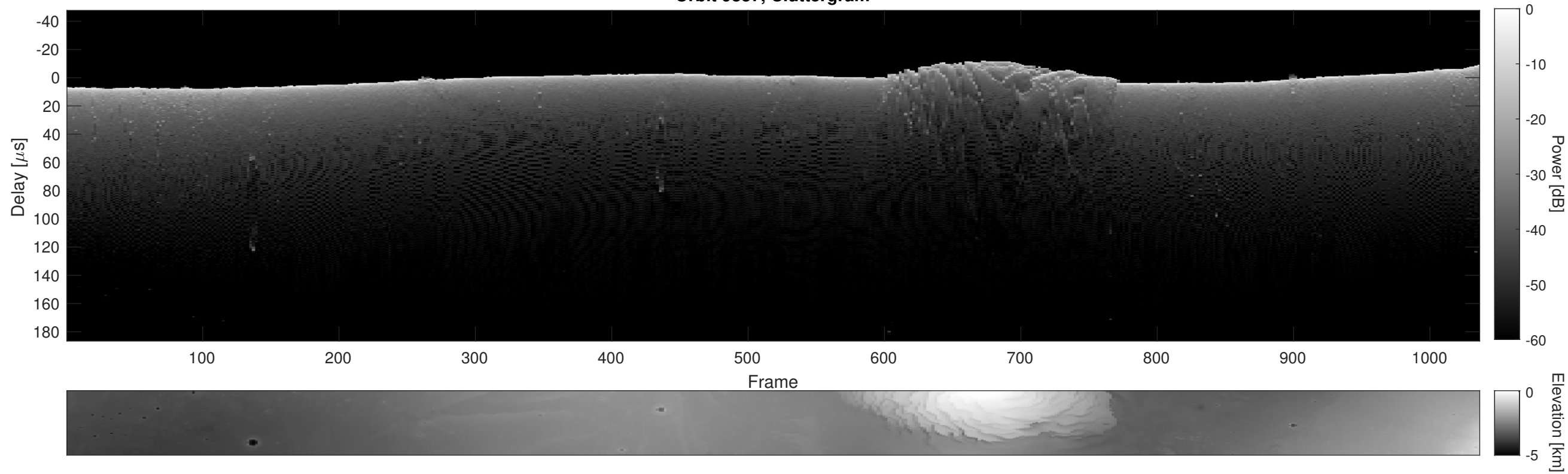
Orbit 9837, Cluttergram
